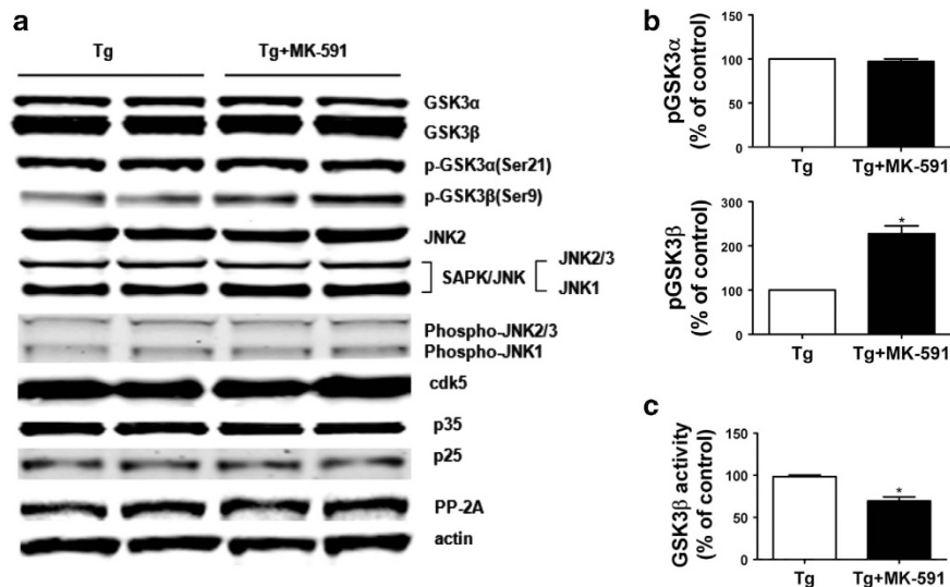
Figure 3. Pharmacologic blockade of 5-lipoxygenase-activating protein (FLAP) reduces glycogen synthase kinase-3β (GSK-3β) activity. (a) Representative western blot analysis for GSK-3α, GSK-3β, pGSK-3α, pGSK-3β, JNK2, SAPK/JNK, p-JNK1, p-JNK2/3, cyclin kinase-5 (cdk5), p35, p25 and PP-2A in brain cortex homogenates from Tg2576 mice receiving MK-591 or vehicle (control). (b) Densitometric analyses of the immunoreactivities to the antibodies shown in the previous panel. (c) Ex vivo GSK-3β activity in brain cortex homogenates of Tg2576 receiving MK-591 or control ( *P = 0.02 ). Results are mean \pm s.e.m.
