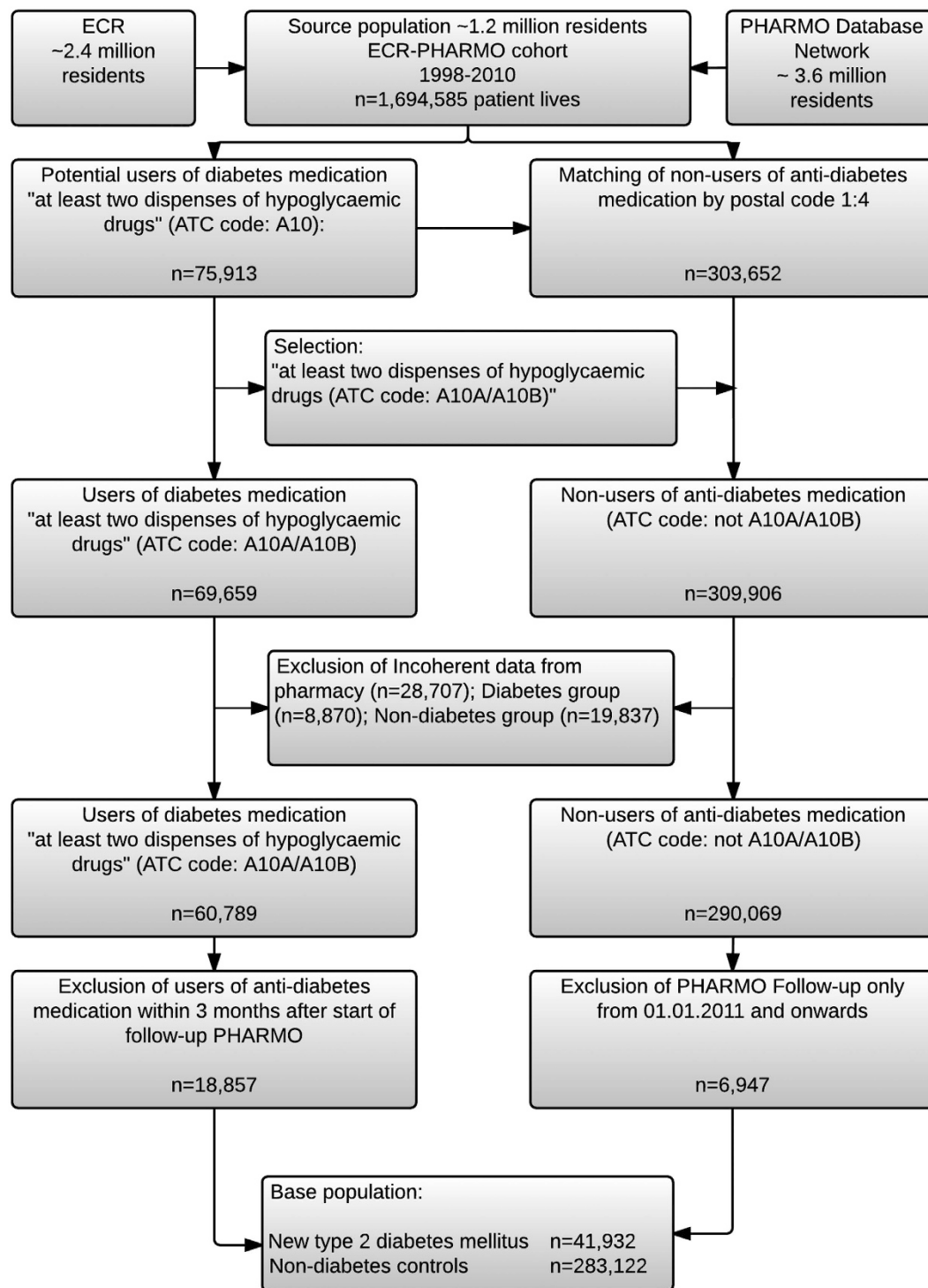
Figure 1. Study flowchart.
