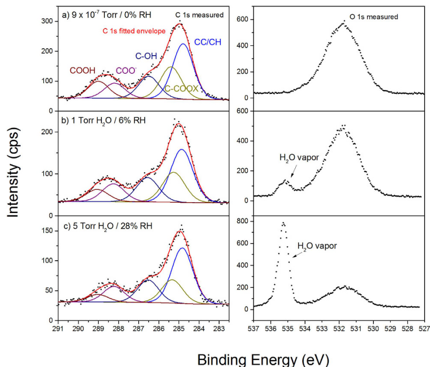
Figure 1. C 1s (left) and O 1s (right) APXPS spectra of an ultrathin PAA film on native aluminum oxide at varying water vapor pressures. 9 \times 10^{-7} Torr (a), 1 Torr H 2 O (b), 5 Torr H 2 O (c).
