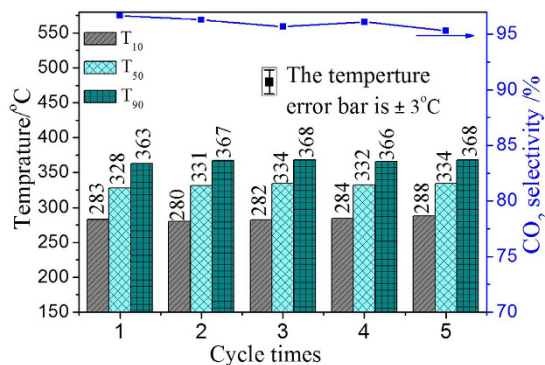
Figure 11. Tested stability results of 3DOM K-OMS-2/SiO 2 -50 catalyst for soot combustion (The temperature error bar is ± 3°C).
