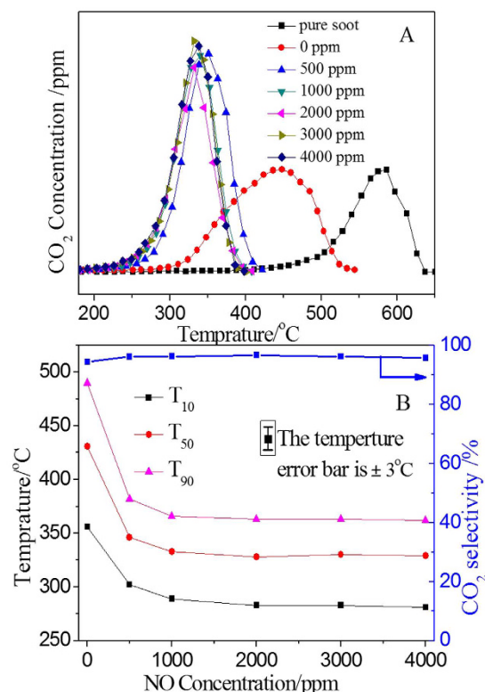
Figure 10. The CO 2 concentration profiles (A) and catalytic activities (B) of K-OMS-2/SiO 2 -50 under different concentrations of NO (The temperature error bar is ± 3°C).
