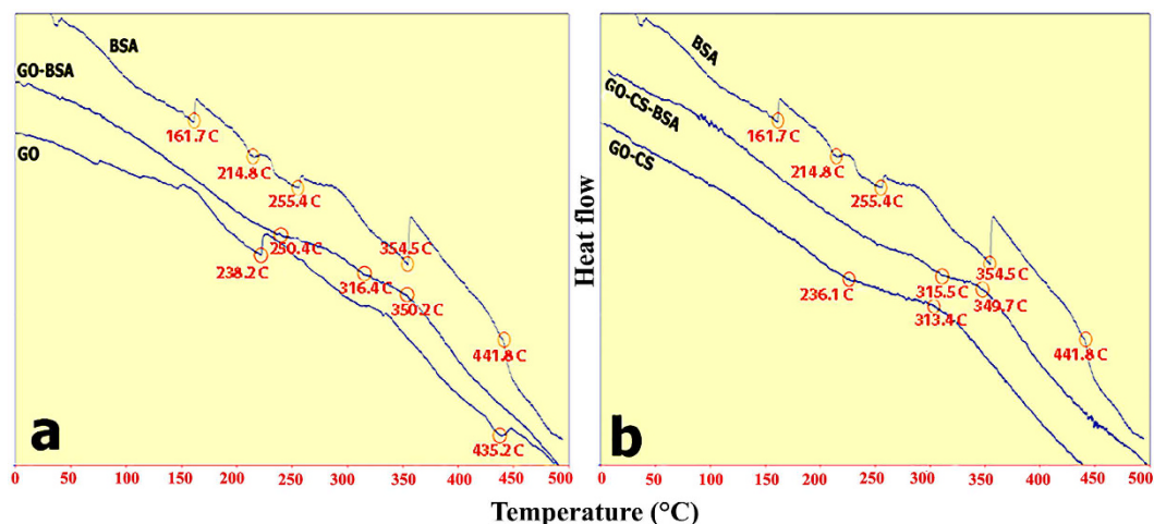
Figure 10. DCS spectra of GO, GO-CS, BSA, GO-BSA, and GO-CS-BSA at a heating rate of 10^{\circ}\text{C min}^{-1} from 40 to 500^{\circ}\text{C} .
