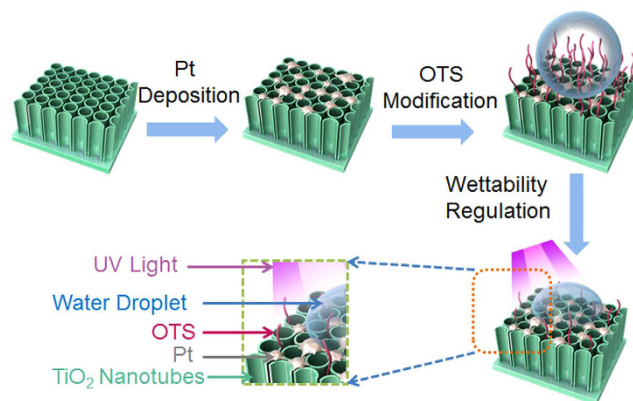
Figure 1. Flow chart for the fabrication and wettability regulation of nanotubular \text{TiO}_2 supported Pt electrodes (Pt- \text{TiO}_2 -NTs). Pt catalysts were deposited on the surface of anodized \text{TiO}_2 nanotubes ( \text{TiO}_2 -NTs) by photocatalytic reduction, which was followed by hydrophobization with vaporized octadecyltrimethoxysilane (OTS) molecules. The wettability of Pt- \text{TiO}_2 -NTs was subsequently regulated in situ from hydrophobicity to hydrophilicity using ultraviolet (UV) light.
