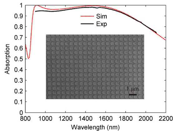
Figure 2. The simulated (red dashed line) and experimental (black solid line) absorption spectra for the fabricated sample. The inset shows the SEM image of a section of the sample.
