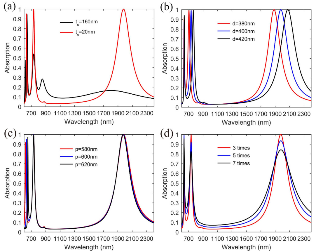
Figure 6. Simulated absorption performance of the Au-disk narrowband absorber. (a) Absorption spectra with different dielectric thickness t_s . The other geometric parameters are p = 600\text{ nm} , d = 400\text{ nm} , t_m = 30\text{ nm} and d_m = 100\text{ nm} . (b) Absorption spectra with different diameter d while other geometric parameters are fixed. (c) Absorption spectra with different period p while other geometric parameters are fixed. (d) Absorption spectra with different damping constants while the geometric parameters are fixed.
