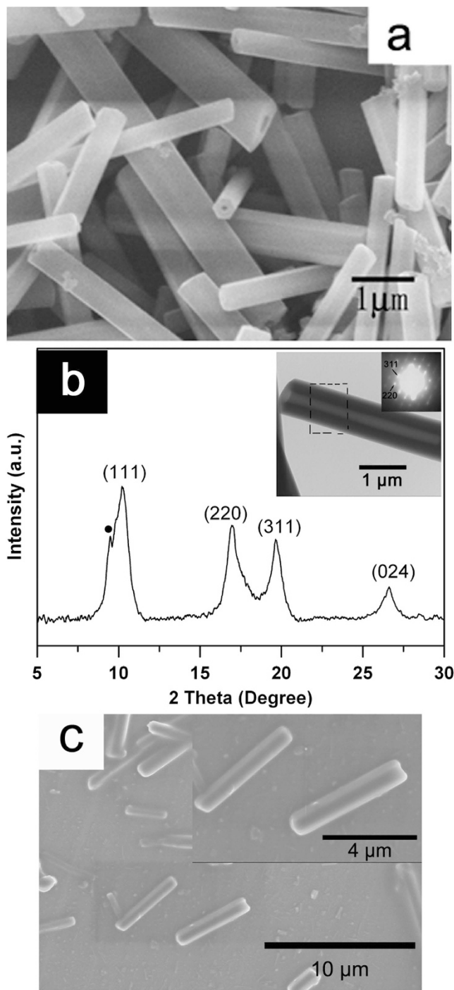
Figure 1. SEM image (a) and XRD pattern (b) of as-grown C 70 nanocrystals, and SEM image of C 70 nanocrystals after treatment under 2.0 GPa, 700 K (c). The insert in figure b shows the TEM image and SAED pattern of a single pristine C 70 nanotube.
