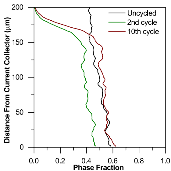
Figure 6. Sulfur phase fraction as a function of thickness of the electrode where 0 μm represents the current collector position.
