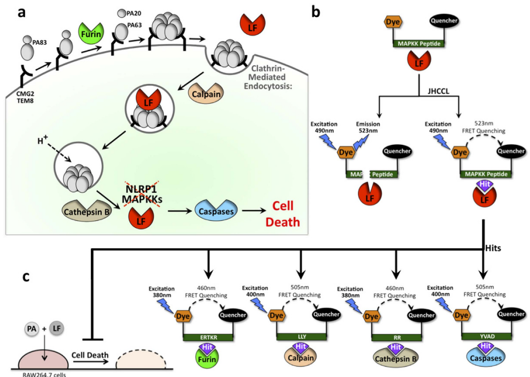
Figure 1. The use of the Johns Hopkins Clinical Compound Library (JHCCl) to screen for inhibitors of anthrax lethal toxin and host proteases. (a) Schematic depiction of host protease components within the pathway that mediates the delivery of anthrax toxin into cytoplasm. Lethal factor (LF) interact with a second B. anthracis protein, protective antigen (PA), whose role is to bind to host cell receptors, CMG2 and TEM8. Three host cell proteins furin, calpain, and cathepsin B mediate the endocytosis of the toxin complex. Once in the cytoplasm, LF cleaves host MAPKK's and NLRP1, and initiates apoptosis through induction of proteolytic activity of host caspases-1 and -3. (b,c) Overall approach scheme: JHCCl is screened by biochemical FRET assay looking for drugs that are able to reduce proteolytic activities of anthrax toxin and five host proteases that mediate toxin lethality. (b) Schematic diagram of FRET screen to identify drugs that inhibit proteolytic reaction of LF, (c) followed by FRET reactions to test the ability of LF inhibitors to also inhibit proteolytic reactions mediated by host furin, calpain, cathepsin B, caspase-1, and caspase-3. In addition, LF FRET inhibitors are tested for their ability to reduce LF-PA cytotoxicity of mouse macrophage cells.
