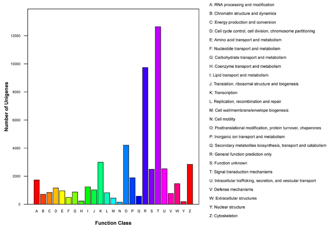
Figure 3. KOG classifications of all unigenes from posterior intestine of M. anguillicaudatus .
