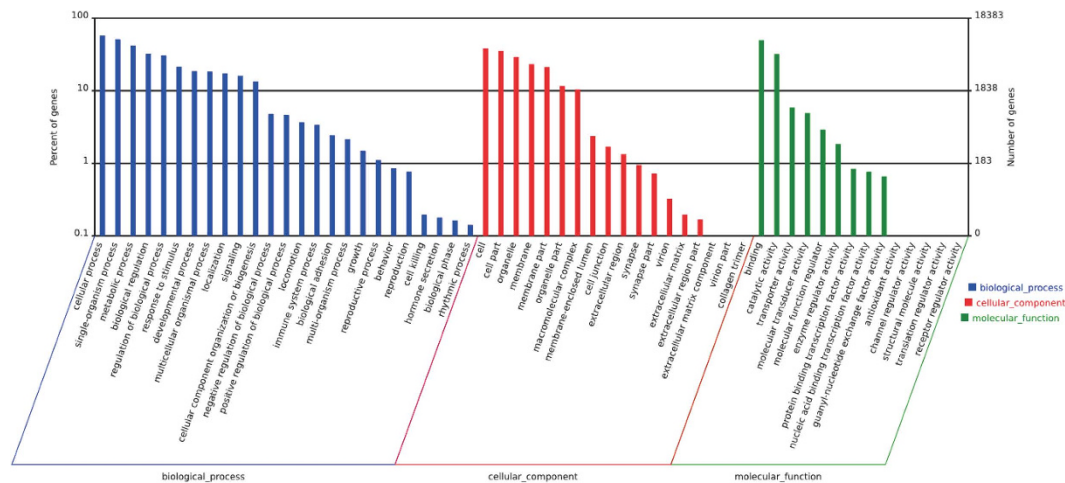
Figure 2. GO classifications of all unigenes from posterior intestine of M. anguillicaudatus .
