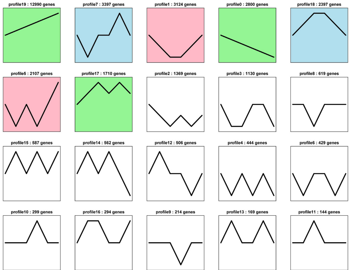
Figure 4. Expression profiles and clusters of DEGs obtained from the STEM clustering. Numbers indicated profiles or gene numbers. Significantly different profiles were represented by different background colors.
