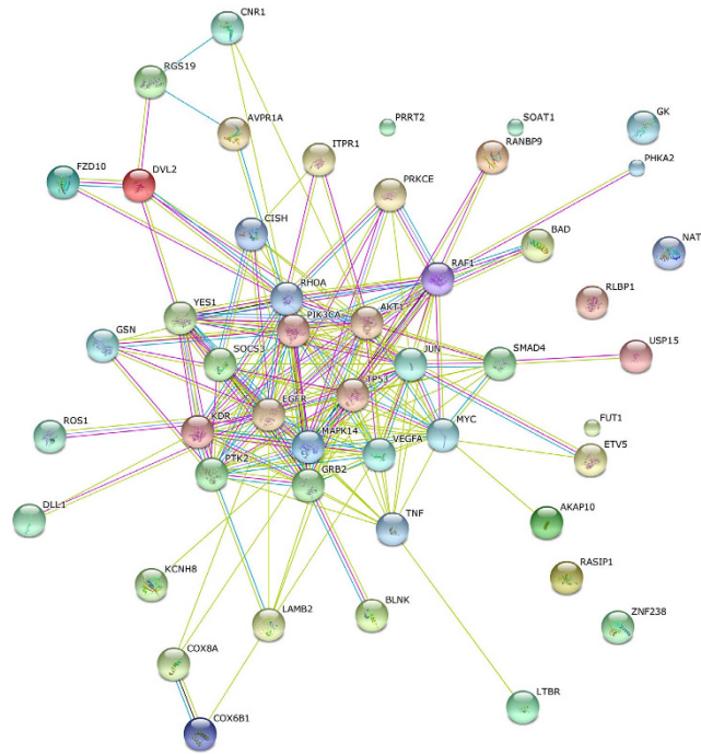
Figure 5. Protein-protein interaction network for the 50 important enzymes encoded by key DEGs of key pathways. Different nodes represented different enzymes. The interactions among these enzymes were represented by different colorful lines.
