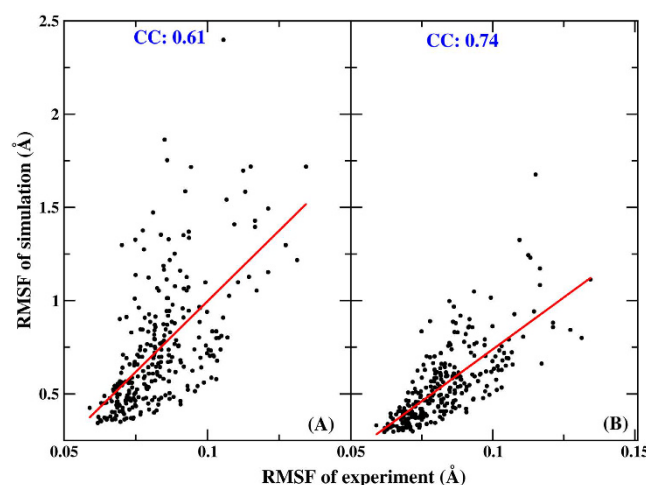
Figure 2. (A) The correlation of the C \alpha RMSF values between X-ray experimental data and the AMBER calculated result. (B) The correlation of the C \alpha RMSF values between X-ray experimental data and the PPC calculated result. CC denotes the correlation coefficient.
