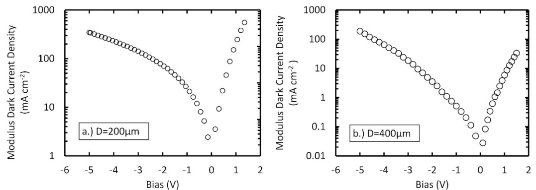
Figure 2. Dark current density as a function of the applied bias; (a) 200 \mu\text{m} diameter, 6 \mu\text{m} epilayer and (b) 400 \mu\text{m} diameter, 0.5 \mu\text{m} epilayer.
