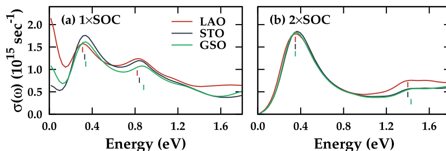
Figure 5. Calculated optical conductivities for \text{SrIrO}_3 (113). Cases with (a) normal ( 1 \times \text{SOC} ) and (b) doubled SOC term ( 2 \times \text{SOC} ) on different substrates. At the peak positions, small vertical lines are drawn for the guide to the eyes.
