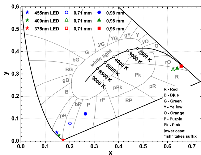
Figure 11. Fragment of the CIE 1931 colour diagram. The colour points of \text{Y}_2\text{Mo}_4\text{O}_{15}:\text{75\%Eu}^{3+} ceramics combined with 375, 400, and 455 nm LEDs. Stars, open, and filled symbols denote colour points of LEDs, LEDs with 0.71 mm ceramic disk, and LEDs with 0.98 mm ceramic disk, respectively.
