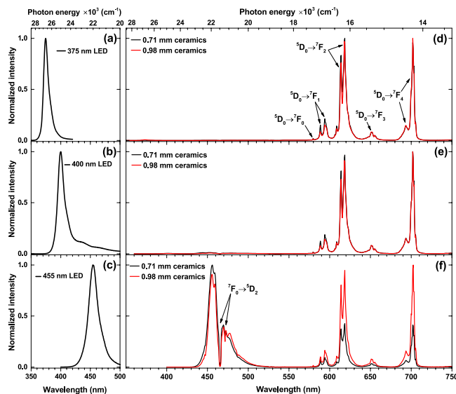
Figure 10. Emission spectra of LEDs and ceramics. (a) 375 nm LED, (b) 400 nm LED, and (c) 455 nm LED. Emission spectra of \text{Y}_2\text{Mo}_4\text{O}_{15}:\text{75\%Eu}^{3+} ceramic disks excited with (d) 375 nm LED, (e) 400 nm LED, and (f) 455 nm LED.
