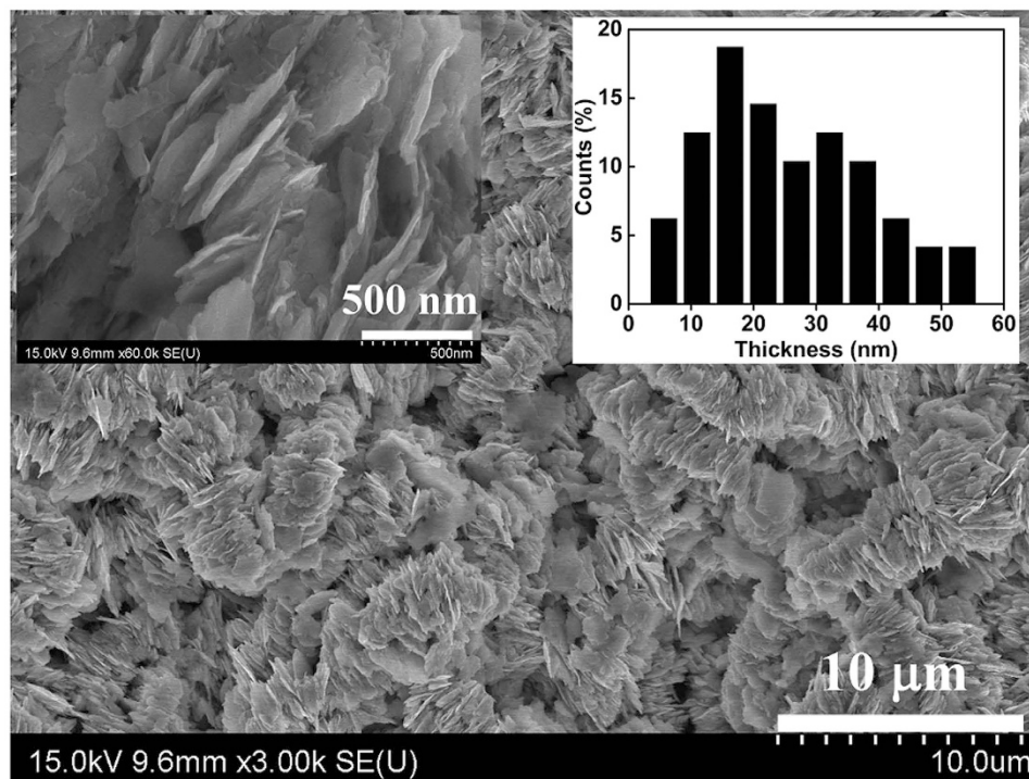
Figure 2. The SEM image of \text{SmCo}_5 nanoflakes milled for 20 h, the top left and top right are the enlarged image and histogram for selected area, respectively.
