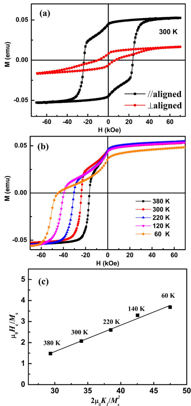
Figure 4. (a) The hysteresis loop, (b) temperature dependence of demagnetization curves and (c) \mu_0 H_c / M_s against 2K_f \mu_0 / M_s^2 on different temperature for aligned \text{SmCo}_5 nanoflakes resin composite.
