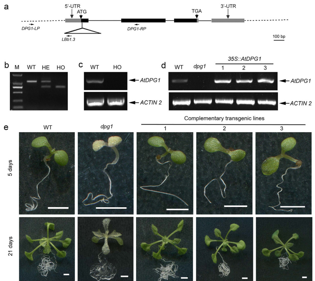
Figure 2. Molecular identification and phenotype rescue of the dpg1 mutant. (a) Gene structure of At1g49510 and the position of the T-DNA insertion. Exons and introns are represented by boxes and lines, respectively. The insertion site of the T-DNA in dpg1 is indicated by a triangle. DPG1-LP , DPG1-RP and LbB1.3 are the primers that were used for genotyping PCR. (b) A representative genotyping PCR result of dpg1 . Offspring of the heterozygous dpg1 were segregated into three genotypes: wild type (WT), heterozygous (HE) and homozygous (HO). (c) Semi-quantitative RT-PCR analysis of AtDPG1 in the wild type (WT) and homozygous dpg1 mutant (HO). The ACTIN2 gene was used as an internal control. (d) Semi-quantitative RT-PCR analysis of the AtDPG1 transcription levels in the wild type (WT), the homozygous dpg1 and three complementary transgenic lines (Lines 1, 2 and 3). The ACTIN2 gene was used as an internal control. (e) The phenotype of a dpg1 homozygous plant was rescued by transformation with a 35S::AtDPG1 transgene. Scale bar = 2 mm.
