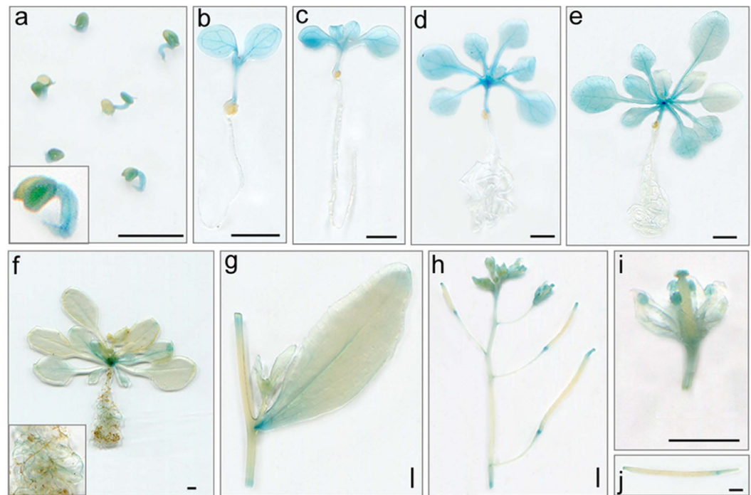
Figure 5. Histochemical assays for the expression pattern of AtDPG1::GUS transgenic lines as visualized by GUS staining. (a) Germinating seeds (36 h after sowing). (b) 5-day-old seedling. (c) 7-day-old seedling. (d) 14-day-old plant. (e) 21-day-old plant. (f) 35-day-old plant. (g) Stem and cauline leaf. (h) Inflorescence. (i) Fully opened flower. (j) Silique. Scale bar = 2 mm.
