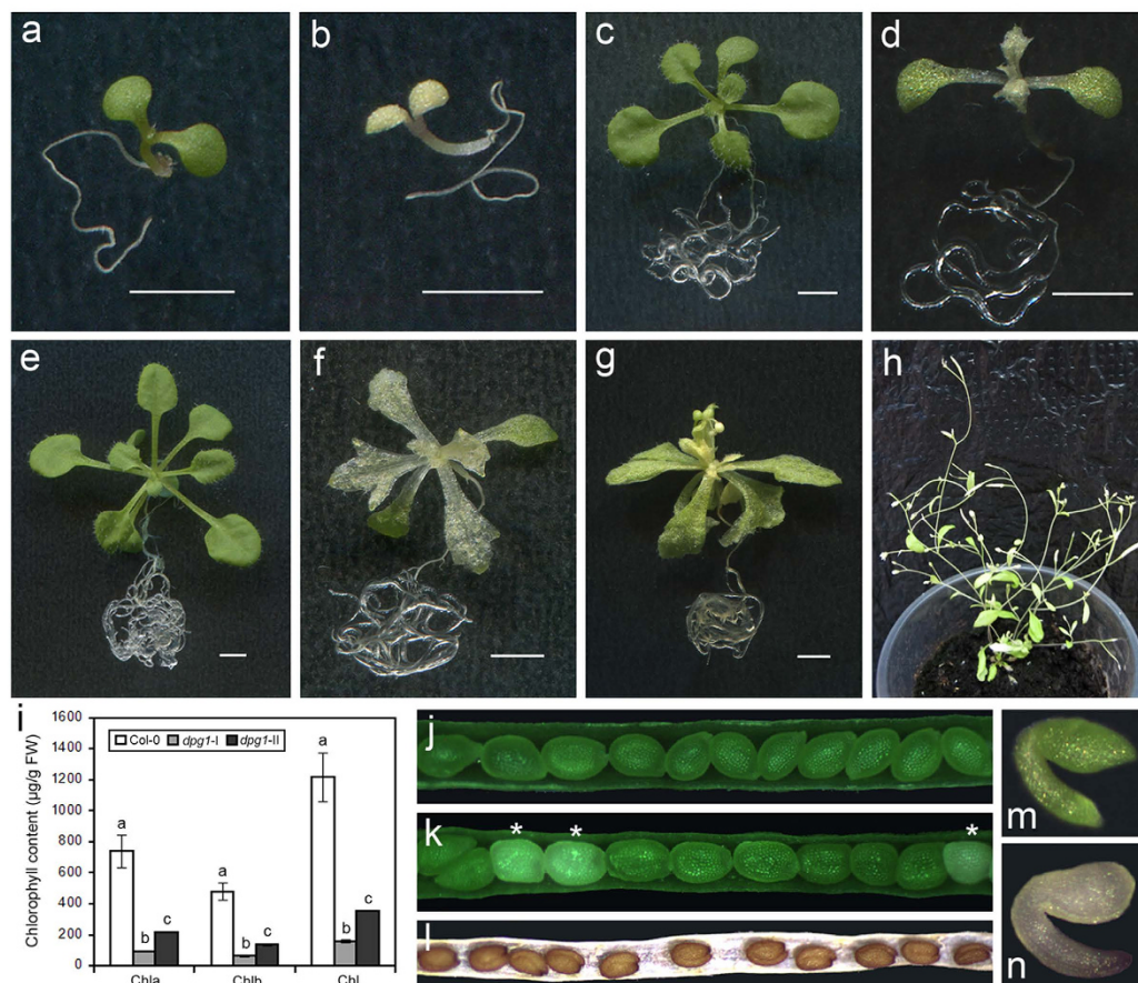
Figure 1. Phenotypic analysis of the dpg1 mutant plants. (a) 5-day-old wild type. (b) 5-day-old dpg1 . (c) 14-day-old wild type. (d) 14-day-old dpg1 . (e) 21-day-old wild type. (f) 21-day-old dpg1 . (g) 35-day-old dpg1 . (h) 90-day-old dpg1 . Scale bar = 5 mm. (i) The chlorophyll contents in the leaves of 21-day-old wild-type (Col-0), 21-day-old dpg1 ( dpg1 -I) and 35-day-old dpg1 ( dpg1 -II) plants. Chla, chlorophyll a; Chlb, chlorophyll b; Chl, total chlorophyll. Each value is the mean \pm SE of three independent determinations, and different letters indicate significant differences at P < 0.05 . (j) Green seeds in a 9-day-old wild-type silique. (k) Intermixed albino and green seeds in a 9-day-old dpg1 heterozygous silique. The asterisks indicate albino seeds. (l) Seeds in a 15-day-old dpg1 heterozygous silique. (m) A representative green embryo in a 9-day-old wild-type silique. (n) A representative albino embryo in a 9-day-old dpg1 heterozygous silique.
