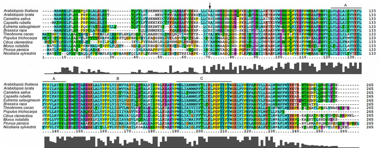
Figure 4. Multiple sequence alignment of AtDPG1 and its homologues. The transmembrane domains (A–C) that were conserved among the DPG1 homologues are indicated. Protein sequences of DPG1 homologues from Arabidopsis lyrata (XP_002891514), Camelina sativa (XP_010479384), Capsella rubella (XP_006304157), Eutrema salsugineum (XP_006393250), Brassica rapa (XP_009124376), Theobroma cacao (XP_007042342), Populus trichocarpa (XP_006384460), Citrus clementina (XP_006423083), Morus notabilis (XP_010096165), Prunus persica (XP_007201809), and Nicotiana sylvestris (XP_009792237) were retrieved from GenBank. The downward arrow indicates the putative cleavage site of the transit peptide of AtDPG1 as predicted by ChloroP 1.1 program. Sequences were aligned with ClustalX 2.0 software.
