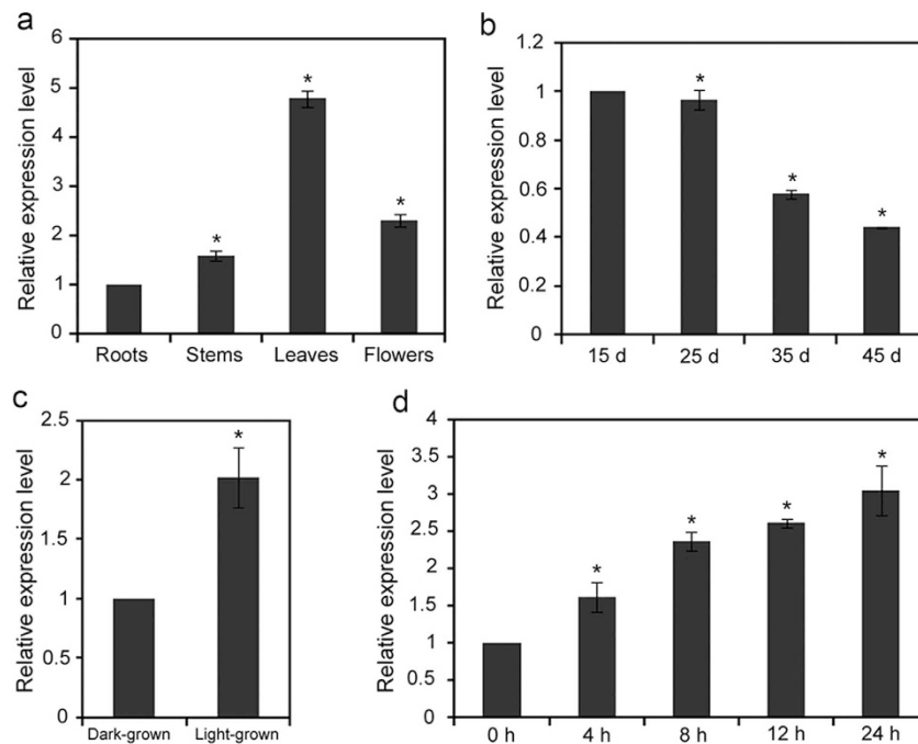
Figure 6. Expression pattern of the AtDPG1 gene. (a) Quantitative real-time PCR analysis of AtDPG1 transcripts in different organs (roots, stems, leaves, and flowers) from 45-day-old wild-type Arabidopsis plants. The expression levels of AtDPG1 displayed a range of cycle C_t values ranging from 22.80 to 24.44 in different tissues. The roots expressed the lowest levels of AtDPG1 mRNA, with a C_t value of 24.44, and the AtDPG1 transcript level in roots was set to 1.0. (b) AtDPG1 transcript levels in the leaves of different developmental stages in wild-type Arabidopsis plants. The AtDPG1 transcript level in the leaves from 15-d-old seedlings was set to 1.0. (c) Transcript levels of AtDPG1 in 4-day-old wild-type light-grown and dark-grown seedlings. The AtDPG1 transcript level in the dark-grown seedlings was set to 1.0. (d) Transcript levels of AtDPG1 during the light-induced greening of etiolated wild-type seedlings. After growth in darkness for 4 days, the etiolated Arabidopsis seedlings were illuminated for 4, 8, 12, and 24 h. The AtDPG1 transcript level in the etiolated seedlings was set to 1.0. The bar graphs show the relative expression levels, as determined by the comparative C_T method and normalized to the expression of the ACTIN2 gene. The error bars indicate the interval delimited by 2^{-(\Delta\Delta C_T \pm SD)} . The asterisks indicate \Delta C_T values significantly different from those of the control in a Mann–Whitney U-test ( P < 0.05 ).
