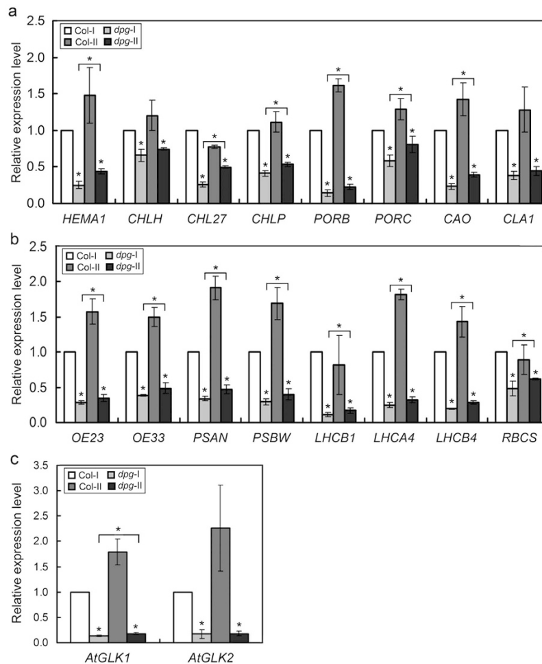
Figure 8. Effects of the AtDPG1 mutation on the expression of nuclear-encoded photosynthetic genes. (a) The expression levels of nuclear-encoded genes that are critical for chlorophyll biosynthesis ( HEMA1 , CHLH , CHL27 , CHLP , PORB , PORC , CAO , and CLA1 ). (b) The expression levels of nuclear-encoded photosynthetic genes ( OE23 , OE33 , PSAN , PSBW , LHCb1 , LHCA4 , LHCb4 , and RBCS ). (c) The expression levels of nuclear-encoded GLK transcription factor genes ( AtGLK1 and AtGLK2 ). The terms dpG1-I and dpG1-II refer to the leaves that were albino or pale-green in 21-day-old and 35-day-old dpG1 mutants, respectively. The transcript level of each gene was set to 1.0 in the leaves from a 21-d-old wild type plant. The bar graphs show the relative expression levels, as determined by the comparative C_T method and normalized with the expression of the ACTIN2 gene. The error bars indicate the interval delimited by 2^{-(\Delta\Delta C_T \pm SD)} . The asterisks indicate \Delta C_T values significantly different from those of control in a Mann–Whitney U-test ( P < 0.05 ).
