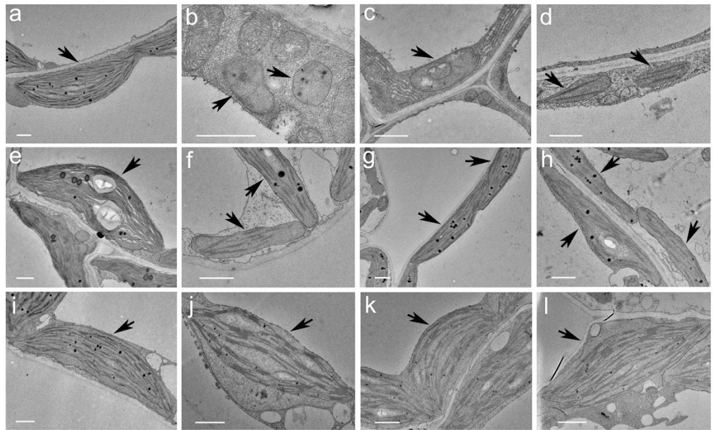
Figure 3. Ultrastructure of chloroplasts from wild-type, dpg1 and complementary plant leaves. (a–d) Chloroplast structures from 21-day-old wild-type (a) and dpg1 (b–d) plants. (e–h) Chloroplast structures from 35-day-old wild-type (e) and dpg1 (f–h) plants. (i–l) Chloroplast structures from 21-day-old wild-type (i) and complementary (j–l) plants. The arrowheads indicate chloroplasts in the wild type, dpg1 and complementary plants. Scale bar = 1 \mu m.
