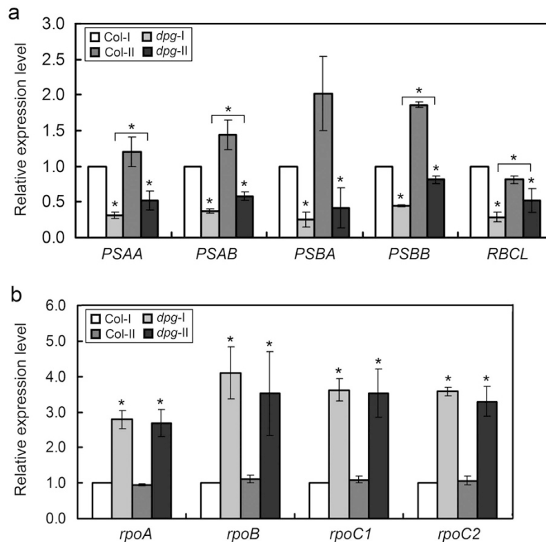
Figure 7. Effects of the AtDPG1 mutation on the expression of chloroplast-encoded genes. (a) The expression levels of chloroplast-encoded PEP-dependent genes ( PSAA , PSAB , PSBA , PSBB , and RBCL ). (b) The expression levels of genes encoding PEP core subunits ( rpoA , rpoB , rpoC1 , and rpoC2 ). The terms dpG1 -I and dpG1 -II refer to the leaves that were albino or pale-green in 21-day-old and 35-day-old dpG1 mutants, respectively. The transcript level of each gene was set to 1.0 in the leaves from a 21-day-old wild type plant. The bar graphs show the relative expression levels, as determined by the comparative C_T method and normalized to the expression of the ACTIN2 gene. Error bars indicate the interval delimited by 2^{-(\Delta\Delta C_T \pm SD)} . The asterisks indicate \Delta C_T values significantly different from those of the control in a Mann–Whitney U-test ( P < 0.05 ).
