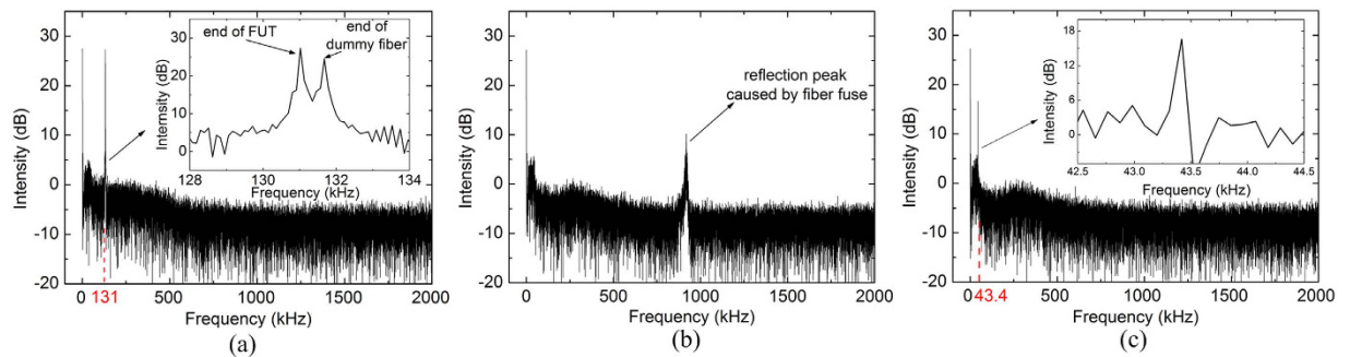
Figure 3. OFDR traces of the FUT: (a) before the fibre fuse initiation; (b) during the fibre fuse propagation; (c) after the fibre fuse termination. The beat frequency of Fresnel peaks before and after the fibre fuse initiation are depicted with dotted lines in (a,c), respectively.
