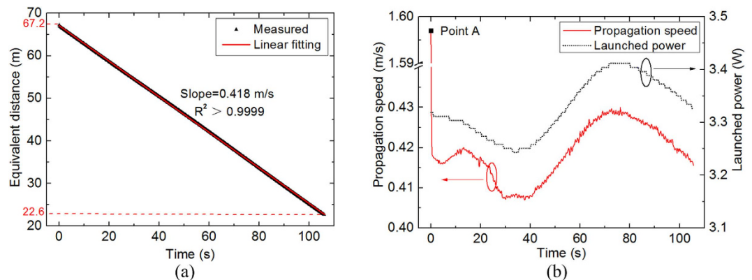
Figure 4. Real-time locating and speed measurement of fibre fuse in a pure silica-core SMF: (a) equivalent distance of the last void as a function of time; (b) fuse propagation speed and launched power as functions of time.
