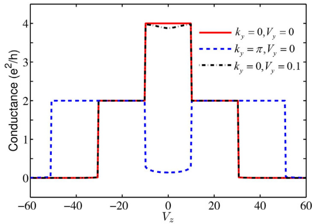
Figure 5. The ZBC for the TSC as a function of the V_z Zeeman field for different values of k_y and V_y . The other parameters for the TSC are the same as in Fig. 1. The parameters in the lead are chosen to be t_L = t , \mu_L = \mu for k_y = 0 , and \mu_L = -\mu for k_y = \pi .
