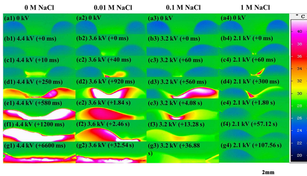
Figure 6. Side-view thermographic pictures of droplets of NaCl solutions with different concentrations (droplet volume: 2 \mu L, droplet separation: 4 mm) on the SR surface under a high positive voltage (the left electrode was energized, and the right one grounded).
