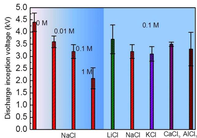
Figure 5. Discharge inception voltages of different salt droplets on the SR surface under a high positive voltage. (Droplet volume: 2 \mu L, the separation between two extreme droplets: 4 mm).
