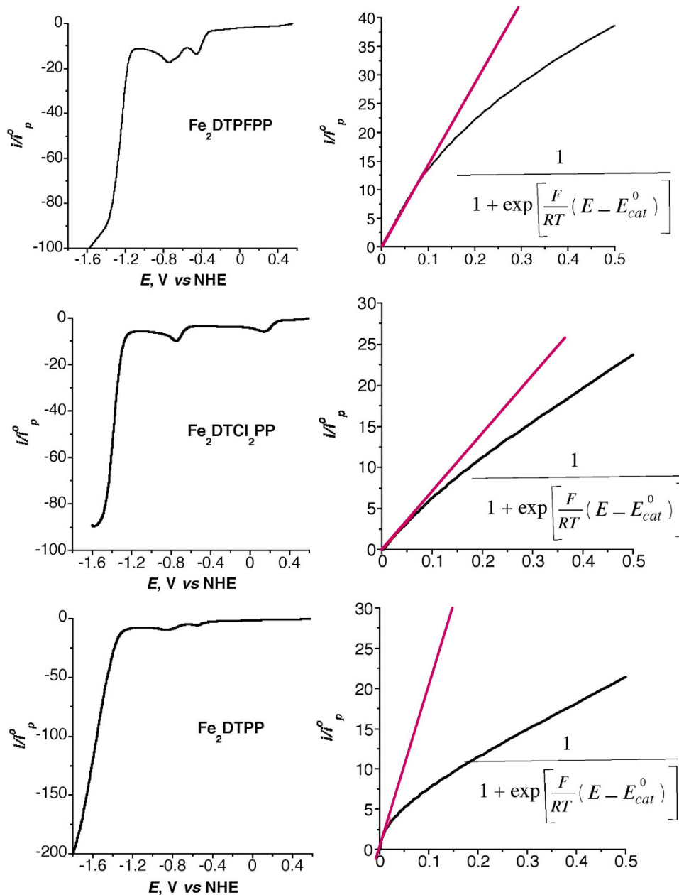
Figure 3. Catalytic CV responses (left, forward scan only shown for clarity) of three Fe porphyrin dimers (0.5 mM) at 100 mV/s scan rate in DMF/10% H 2 O saturated with CO 2 and the corresponding foot-of-the-wave analysis (right).
