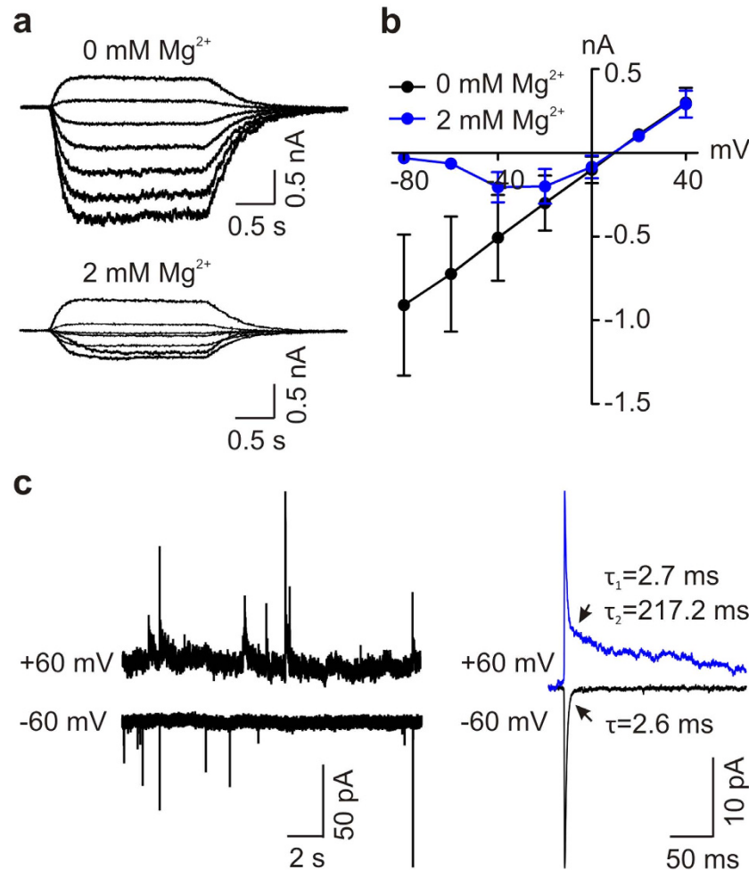
Figure 3. Extracellular Mg 2+ causes voltage-dependent block on NMDA-evoked currents and synaptic NMDAR currents in human iPSC-derived neurons. (a) Representative traces showing agonist-evoked NMDAR currents elicited at a series of membrane potentials from -80 mV to +40 mV (in 20 mV increments) in the absence (upper) and presence (bottom) of 2 mM Mg 2+ in a human iPSC-derived neuron. (b) A plot showing current-voltage relationship of NMDAR currents in the absence and presence of 2 mM Mg 2+ in human iPSC-derived neurons. n = 3 . (c) Left, Typical trace showing mEPSCs recorded at the membrane potentials of -60 mV (bottom) and +60 mV (upper) in presence of extracellular Mg 2+ at 2 mM in a human iPSC-derived neuron. Right, Averaged mEPSCs in this cell at the membrane potentials of -60 mV and +60 mV.
