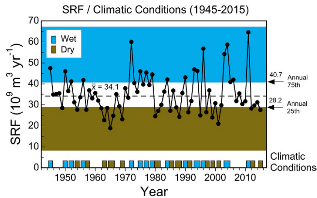
Figure 2. Annual freshwater flow from the Susquehanna River for 1945–2015, indicating dry and wet years based on 25 th and 75 th percentiles.
