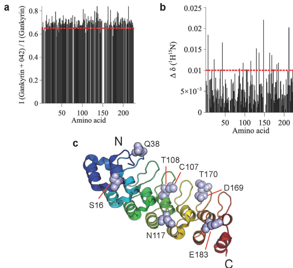
Figure 4. NMR analysis of the gankyrin-cjoc42 interaction. (a) Changes in cross-pipe intensity of the amide backbone of gankyrin in the presence of cjoc42. (b) Changes in chemical shifts of the amide backbone of gankyrin in the presence of cjoc42. (c) Residues 16, 38, 107, 108, 117, 169, 170, 183, with chemical shift changes ( \Delta\delta ( ^{15}\text{N}-^1\text{H} )) of >0.01 that also show significant intensity changes in the presence of cjoc42, are shown on the gankyrin structure.
