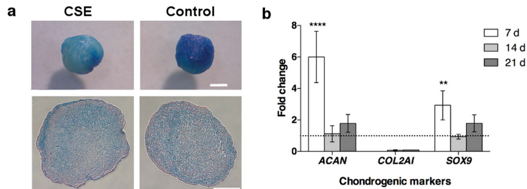
Figure 6. Mucins and gene expression for chondrogenic differentiation. AdMSCs were centrifuged in order to form pellet cultures and induced with chondrogenic supplementation while simultaneously being exposed to 0.5% CSE for 24 h. (A) After 21 d in culture, the pellets were stained with Alcian Blue and sections (5 μm) were further stained with Nuclear Fast Red. A more even stain is observed in the control cell pellets (Scale bar = 1 mm). (B) The gene expression was analysed via a proteoglycan promoter ( ACAN ), structure and strength building proponent ( COL2A1 ), and a chondrogenic transcription factor ( SOX9 ). While the CSE exposed pellets seem to have a much higher expression of ACAN and SOX9 initially, the levels become comparable at later time points. In addition, based on the lack of COL2A1 , CSE exposed pellets would indicate a cartilaginous material with poor extracellular matrix and mechanical function. (** p < 0.01 , **** p < 0.0001 ).
