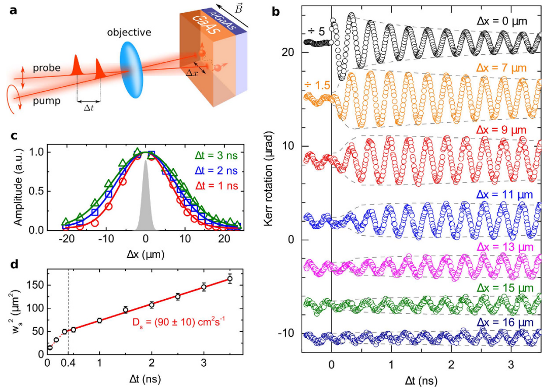
Figure 1. Measurement of the spin life-time and spin diffusion coefficient. (a) A sketch of the spatially resolved pump-and-probe optical experiment. Circularly polarized pump and linearly polarized probe pulses are relatively time-delayed by \Delta t and focused to 2 \mu\text{m} sized spots (full width at half maximum). The spots can be spatially separated by \Delta x by tilting the incident pump beam. The magnetic field B is applied in-plane along the pump-probe separation direction. The sample was kept at temperature 10 K. (b) Kerr rotation dynamics measured by the spatially resolved pump and probe technique for several \Delta x . The \Delta x -dependent increase of the signal in time is a signature of diffusive spin-transport. The non-oscillatory envelopes (gray dashed curves) are calculated from Eq. 1 using the transient D_s^* and intrinsic steady-state D_s for \Delta t < 0.4 ns and \Delta t > 0.4 ns, respectively. The data were vertically shifted and upper two curves were divided by indicated factors for clarity. (c) The spatial Gaussian dependence of the amplitude of the oscillatory Kerr signal at \Delta t = 1, 2 and 3 ns (marked by circles, squares and triangles, respectively) and the corresponding fits using Eq. 1. The spatial profile of the pump spot is depicted by the grey area. (d) \Delta t dependence of the half-width of the spatial Gaussian profile of the amplitude of the oscillatory Kerr signal.
