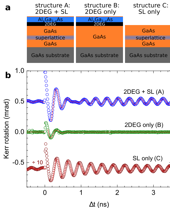
Figure 4. Example of the robustness of the long spin life-time signal in complex heterostructures.
