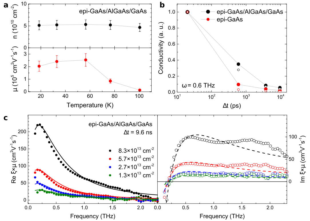
Figure 3. DC and THz transport measurements. (a) DC Hall measurements of the transient carrier mobility and sheet carrier concentration with pulse laser illumination of the Hall cross at wavelength 815 nm and fluence generating a photocarrier density of 4 \times 10^{13} \text{ cm}^{-2} . (b) Time dependence of the representative value of the photoconductivity spectra (imaginary part at \omega = 0.6 \text{ THz} ). Data correspond to photoexcitation at fluence generating a carrier density of 2.6 \times 10^{13} \text{ cm}^{-2} and wavelength 800 nm (closed symbols) and at fluence generating a carrier density of 5.7 \times 10^{13} \text{ cm}^{-2} and wavelength 400 nm (open symbols), and to the GaAs/AlGaAs/GaAs sample (black symbols) and the reference sample containing the GaAs epilayer on the GaAs substrate (red symbols). The photoconductivity at \Delta t = 20 \text{ ps} is normalized to unity. (c) THz spectra of normalized complex photoconductivity as a function of pump photon fluence (i.e. of the density of photocarriers) at 400 nm and time delay 9.6 ns. Lines show fits by the two Drude terms from Eq. 4.
