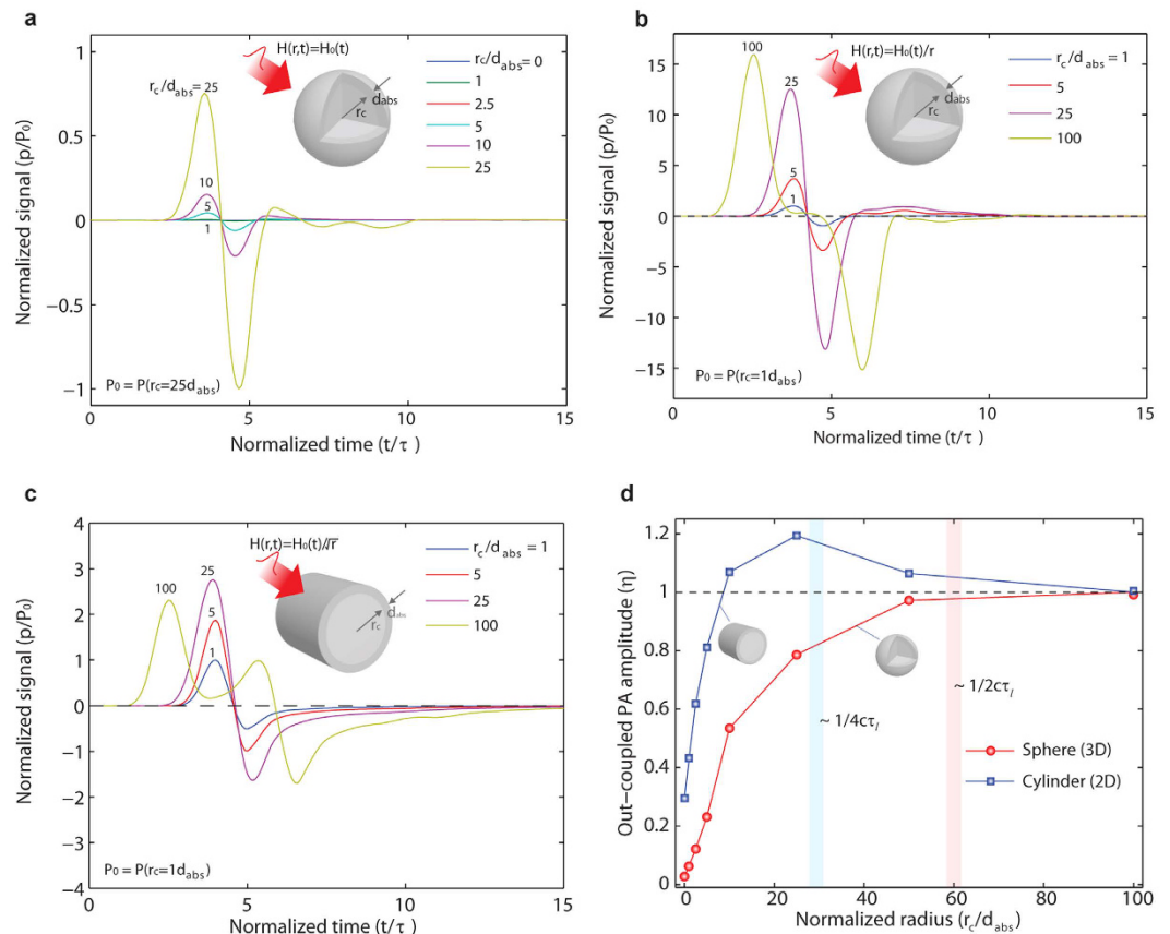
Figure 5. (a) Simulated photoacoustic (PA) signals of a sphere with a transparent core ( r_c ) and an absorbing shell ( d_{abs} ). The transparent core serves as an impedance matching medium analogous to the matching layer for the planar absorber. PA signals are produced by the spatially uniform heating H_0(t) , which is the Gaussian temporal pulse with pulse duration \tau . The PA signals for different matching core radii are obtained at a distance of r_{obs} = r_c + d_{abs} . And the signals are normalized to the pressure amplitude for a sphere with r_c = 1 d_{abs} , i.e., P_0 = P(r_c = 1 d_{abs}) . The resulting signals are due to the combined effect of the PA cancellation and 1/r -decay of spherical waves. (b) PA signals for the scaled heating function H_0(t)/r to only evaluate the cancellation effect. The two PA pulses are completely separated at r_c = 100 d_{op} . (c) Simulated PA signals for a cylinder subject to the scaled heating function H_0(t)/r^{0.5} ( 1/r^{0.5} -decay of cylindrical waves). (d) The out-coupled photoacoustic amplitude ( \eta ) versus the core radius ( r_c ) for spheres and cylinders with the constant shell thickness ( d_{abs} ).
