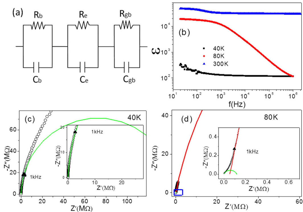
Figure 4. Impedance analysis and dielectric behavior of 10% (In + Nb) co-doped rutile \text{TiO}_2 polycrystalline ceramics. (a) The equivalent electric circuit. (b) Dielectric constant as a function of frequency. (c, d) are Impedance spectroscopy at 40 K and 80 K respectively. The solid symbols are the experimental results. The solid lines are the best fitting results.
