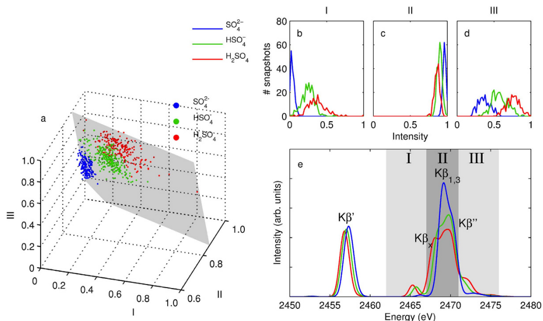
Figure 3. (a) The individual-snapshot spectra presented in a plot of three intensity values I–III for all snapshots of all concentrations. Coloring refers to protonation state of the excited acid molecule and the grey plane presents the best fit using a plane. The values have been normalized to 1 corresponding the maximum. The intensity distributions in regions (b) I, (c) II, and (d) III, with respect to protonation state of the acid molecule. Again, the values are normalized to the maximum intensity of any snapshot in the region. (e) The averaged spectra of the three different forms of acid based on the 600 snapshot total.
