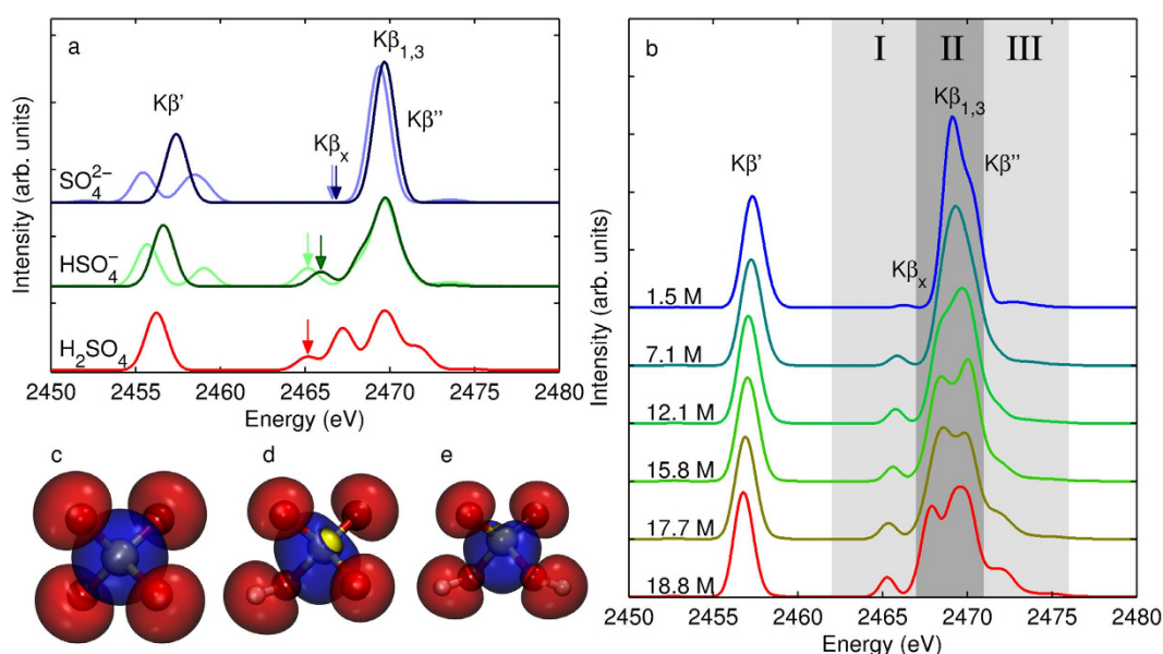
Figure 2. (a) Calculated S K\beta emission spectra of SO_4^{2-} , HSO_4^- , and H_2SO_4 in gas phase. The lighter color represents the spectra of SO_4^{2-} , HSO_4^- without re-optimization of the geometry, and the darker colour represents the spectra with geometry optimization for the particular species. The arrows show the position of the line originating from orbital 14. (b) Calculated S K\beta emission spectra of aqueous sulphuric acid in the range from 1.5 M to 18.8 M, based on ab initio molecular dynamics simulations. The calculated orbital 14 (in the ground state) responsible for lowest transition of the K\beta_x line in the emission spectra of (c) SO_4^{2-} , (d) HSO_4^- , and (e) H_2SO_4 .
