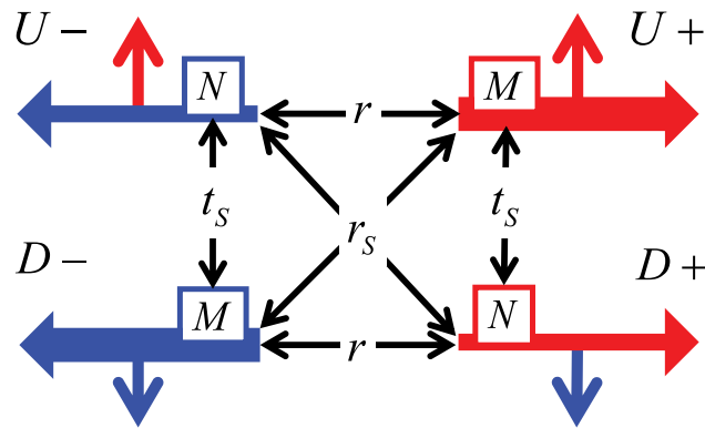
Figure 1. (a) Physical structure: A two dimensional (2D) channel with spin-orbit coupling (SOC).
