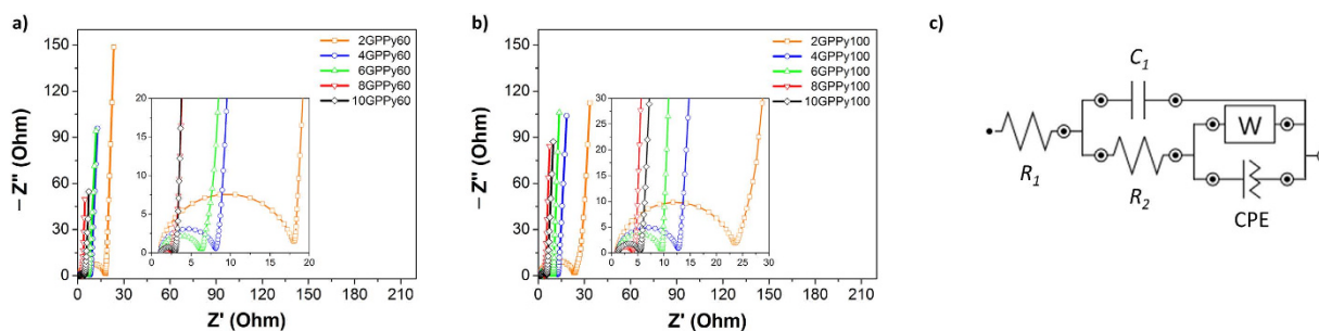
Figure 6. EIS Nyquist plots of the GPPy nano hybrids measured in 1 M sulfuric acid. (a) GPPy60 and (b) GPPy100 samples in the 100 \text{ mHz} to 1 \text{ MHz} frequency range. (c) An equivalent circuit model.
