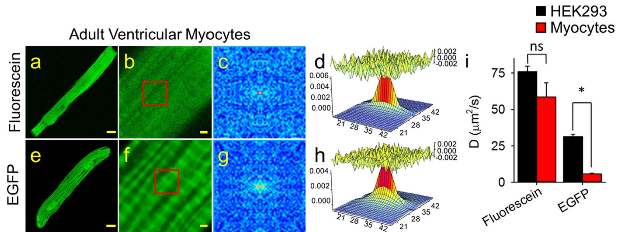
Figure 2. RICS analysis of fluorescein and EGFP in adult ventricular cardiac myocytes. Representative confocal images of fluorescein (a,b) and EGFP (e,f) in myocytes at low (a,e, scale bar 10\mu\text{m} ) and high (b,f, scale bar 1\mu\text{m} ) magnification. (c,g) Average of the spatial correlation calculated for a region of 64 \times 64 pixels (indicated by the red box in b,f) for each of 100 images of fluorescein (c) and EGFP (g) in myocytes. Fit of the correlation functions for fluorescein (d) and EGFP (h). The plot at the top of those panels represents difference between the autocorrelation and the fit. (i) Bar plots (average \pm s.e.m.) of the diffusion coefficient ( D ) values obtained for fluorescein and EGFP in HEK293 cells (black bars) and cardiac myocytes (red bars). * p < 0.05 , ns = not significant. HEK293 cells: n = 4-8 , myocytes: n = 7-22 .
