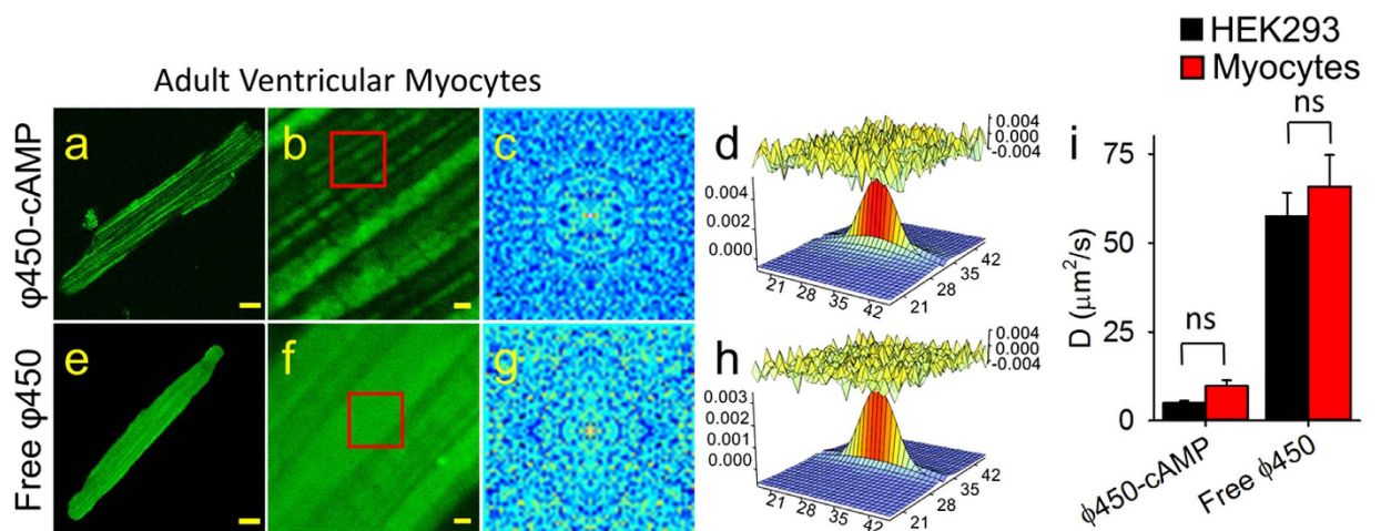
Figure 3. RICS analysis of \phi 450 -cAMP and free \phi 450 in adult ventricular cardiac myocytes. Representative confocal images of \phi 450 -cAMP (a,b) and free \phi 450 (e,f) in myocytes at low (a,e, scale bar 10\mu\text{m} ) and high (b,f, scale bar 1\mu\text{m} ) magnification. (c,g) Average of the spatial correlation calculated for a region of 64 \times 64 pixels (indicated by the red box in b,f) for each of 100 images of \phi 450 -cAMP (c) and free \phi 450 (g) in myocytes. (d,h) Fit of the correlation functions. The plot at the top of those panels represents the difference between the autocorrelation and the fit. (i) Bar plots (average \pm s.e.m.) of the diffusion coefficient ( D ) values obtained for \phi 450 -cAMP and free \phi 450 in HEK293 cells (black bars) and cardiac myocytes (red bars). * p < 0.05 , ns = not significant. HEK293 cells: n = 8-12 , myocytes: n = 9-37 .
