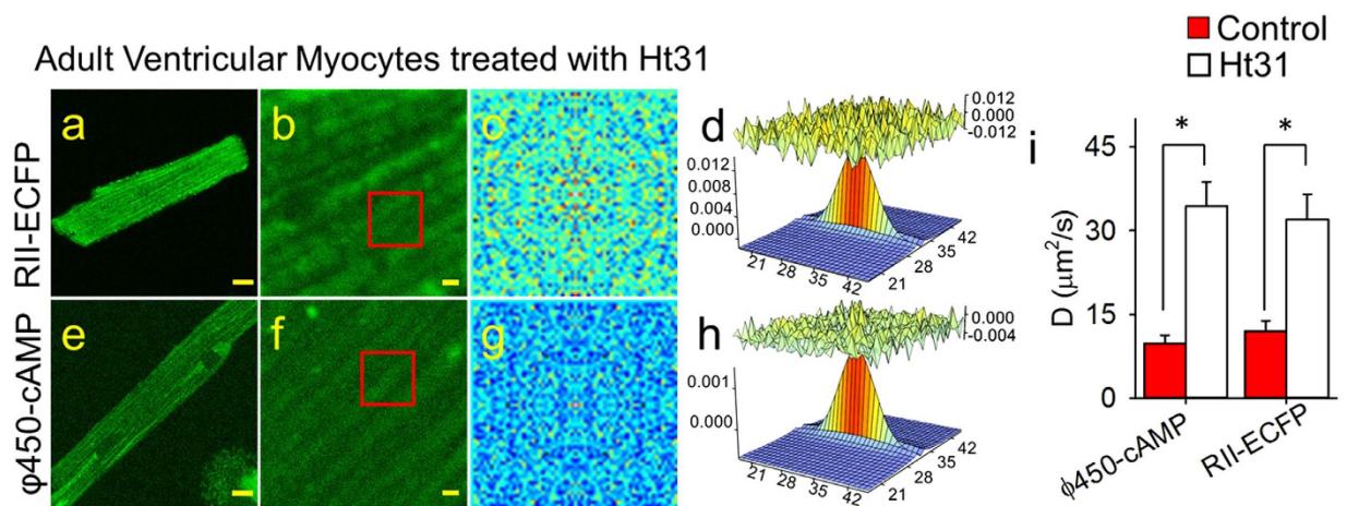
Figure 5. RICS analysis of \phi 450-cAMP and RII-ECFP in adult ventricular cardiac myocytes treated with St-Ht31 peptide. Representative confocal images of St-Ht31-treated myocytes expressing RII-ECFP (a,b) or loaded with \phi 450-cAMP (e,f) at low (a,e, scale bar 10 \mu m) and high (b,f, scale bar 1 \mu m) magnification. (c,g) Average of the spatial correlation calculated for a region of 64 \times 64 pixels (indicated by the red box in b,f) for each of 100 images of RII-ECFP (c) and \phi 450-cAMP (g) in St-Ht31-treated myocytes. Fit of the correlation functions for RII-ECFP (d) and \phi 450-cAMP (h). The plot at the top of those panels represents the difference between the autocorrelation and the fit. (i) Bar plots (average \pm s.e.m.) of the diffusion coefficient ( D ) values obtained for RII-ECFP and \phi 450-cAMP in control (red bars) or St-Ht31-treated (open bars) myocytes (* p < 0.05 . RII-ECFP expressing cells: n = 8-11 , \phi 450-cAMP loaded cells: n = 15-37 ).
