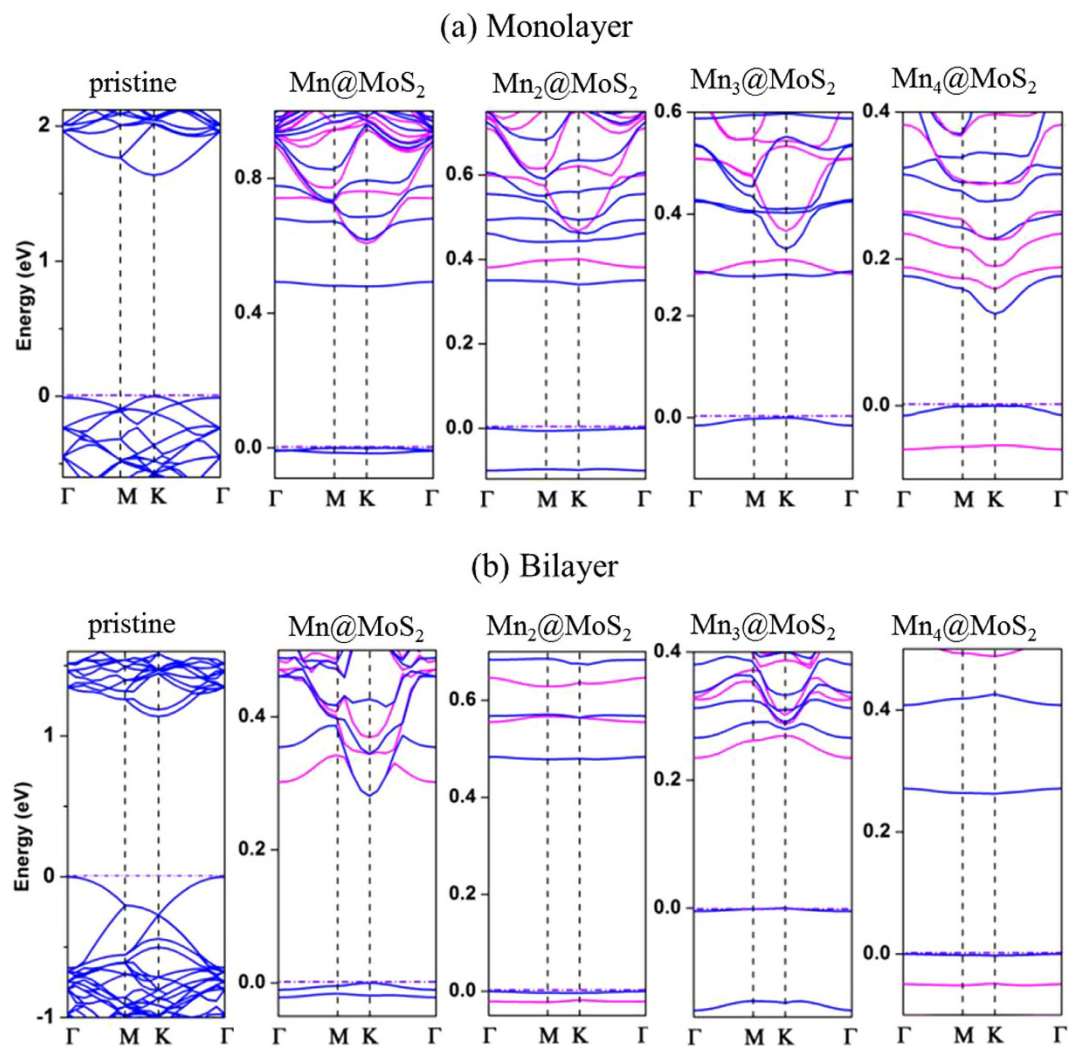
Figure 3. Spin-polarized band structures of the Mn_n adsorbed MoS_2 systems. (a) Band structures of the Mn_n@MoS_2 pizzas. (b) Band structures of the Mn_n@MoS_2 sandwiches. The blue and magenta lines represent the spin-up and spin-down components, respectively. The horizontal dash-dot lines indicate the Fermi level. The band structures of the pristine hosts are depicted at the very left column for comparison purpose.
