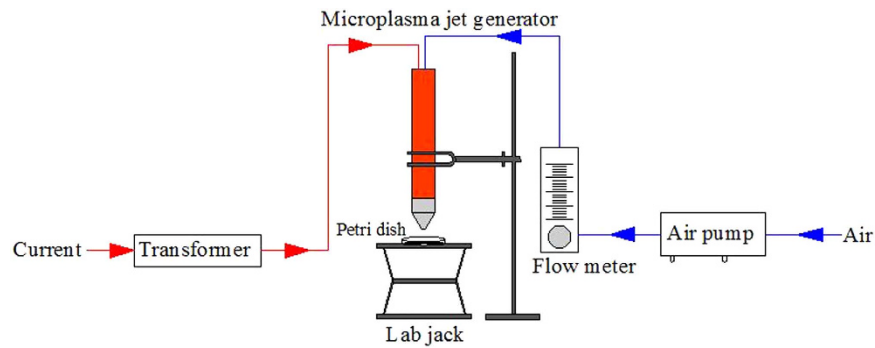
Figure 1. The experimental device: it is mainly composed of the power supply system, gas supply system and the microplasma generation system.
