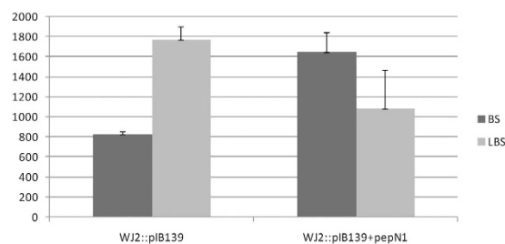
Figure 6. The yield of BS and LBS in S. lividans YGY7 (WJ2::pIB139), S. lividans YGY6 (WJ2::pIB139 + pepN1). The ratio of BS to LBS yield in the YGY6 is 3:2 as compared to that of 1:2 in YGY7, the yield of BS has nearly doubled.
