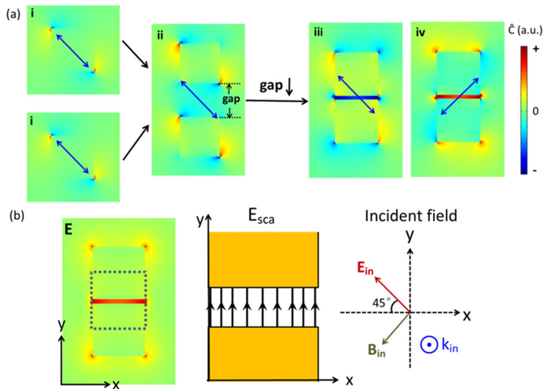
Figure 3. Formation schematic of enhanced chiral near-fields with uniform optical chirality in the gap of a Au block (60 nm × 60 nm × 30 nm) dimer located on glass substrate in water surroundings, excited under polarizations indicated by blue arrows. (a) Chiral near-fields distributions of (i) one Au block, (ii) two blocks with a large gap d of 50 nm, and (iii–iv) block dimers with a small gap d of 5 nm. (b) Corresponding electric fields distribution of the case (a)-iii (left image); the right schematics show directions of incident fields and scattered fields (only fields in the gap are concerned) by a block dimer. All slices are cut from middle positions of the height.
