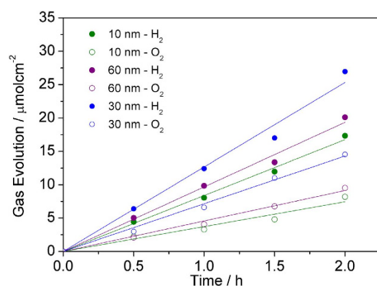
Figure 10. Gas evolution at an applied potential of 0.5 V (vs. Ag/AgCl).
