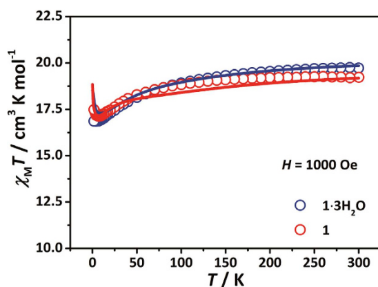
Figure 2. Temperature dependencies of \chi_M T products for 1·3H 2 O and 1 . The temperature range is 1.8 K \leq T \leq 300 K, and the applied field of 1,000 Oe.
