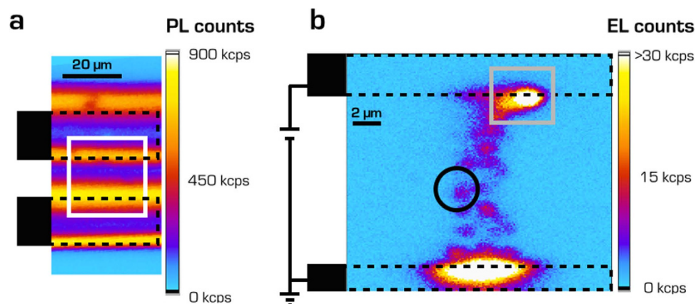
Figure 3. Mapping of luminescent emission. (a) PL map acquired with a \lambda = 532 nm laser excitation from the region highlighted by the black rectangle in Fig. 1b. (b) EL map (215 V bias) from the region highlighted by the white rectangle in Fig. 3a. The dashed black lines indicate the relative position of the electrodes.
