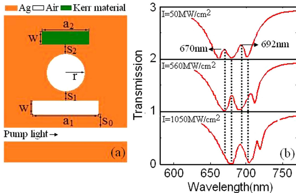
Figure 5. (a) Schematic of the bright-dark-dark plasmonic waveguide with cavity 3 filled with the Kerr nonlinear material. The parameters are S_0 = 20 nm, S_1 = 30 nm, S_2 = 30 nm, W = 50 nm, a_1 = 400 nm, a_2 = 300 nm and r = 165 nm. (b) Transmission spectra of plasmonic waveguide side coupled with Kerr nonlinear resonator as a function of pump light intensity.
