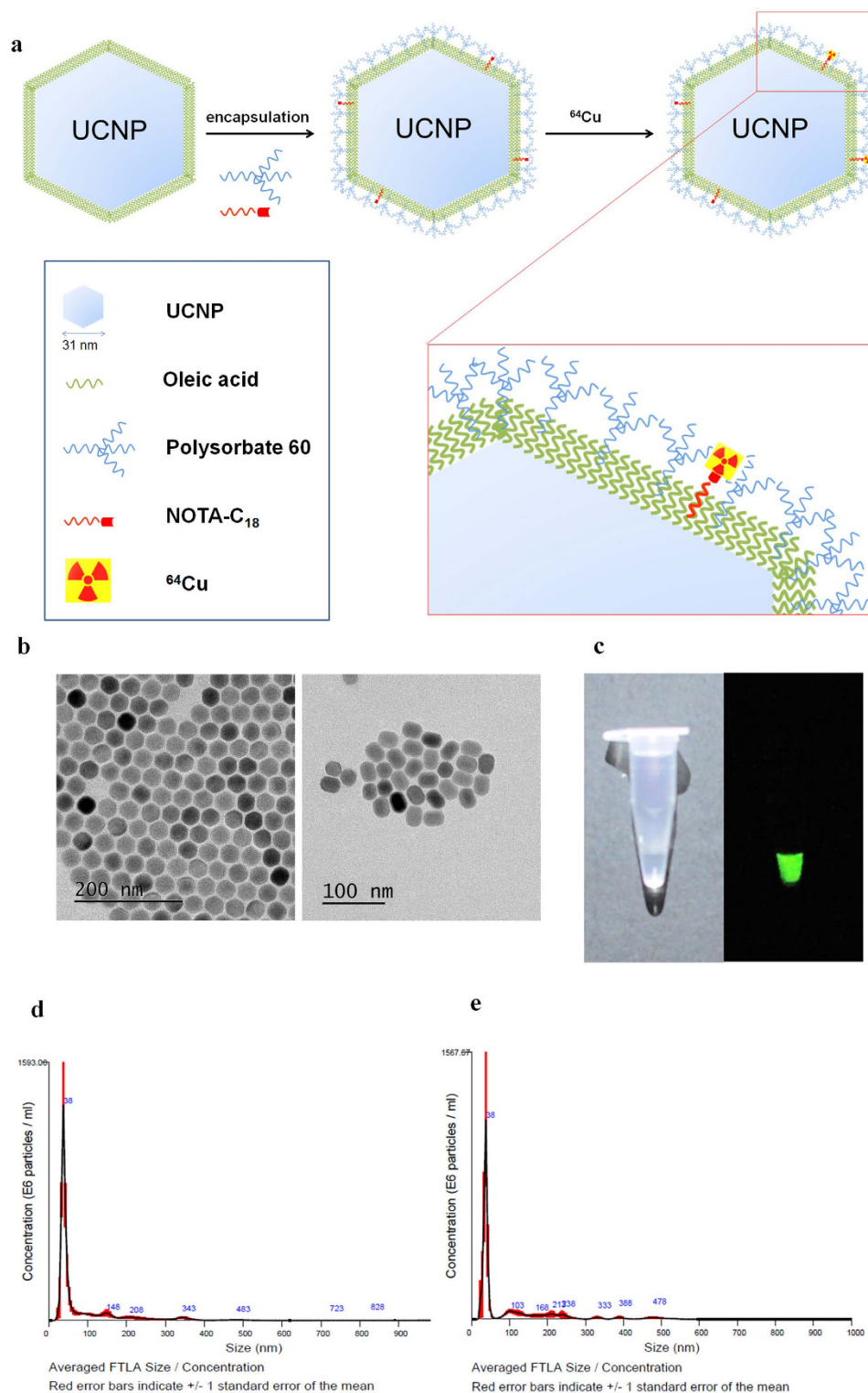
Figure 1. Synthesis and characterization of micelle encapsulated 64 Cu-NOTA-UCNP. (a) Polysorbate 60 was used to transfer the hydrophobic UCNP into aqueous phase and NOTA-C 18 was used for the radiolabeling. Then, 64 Cu was added and labeled with NOTA-UCNPs. Enlarged configuration of micelle encapsulated 64 Cu-NOTA-UCNP was included. Compounds including UCNP, polysorbate 60, NOTA-C 18 , oleic acid and 64 Cu are listed in the blue box. (b) TEM image of UCNP before (left) and after (right) micelle encapsulation (c), Upconversion luminescence image of UCNP under 980 nm laser excitation. (d,e) Size of micelle encapsulated UCNP (d) and micelle encapsulated 64 Cu-NOTA-UCNP (e) measured by nanoparticle tracking analysis (NTA) method showing sharp peak which indicates uniform size of the nanoparticles. Size of micelle encapsulated 64 Cu-NOTA-UCNP showed similar size with the micelle encapsulated UCNP.
