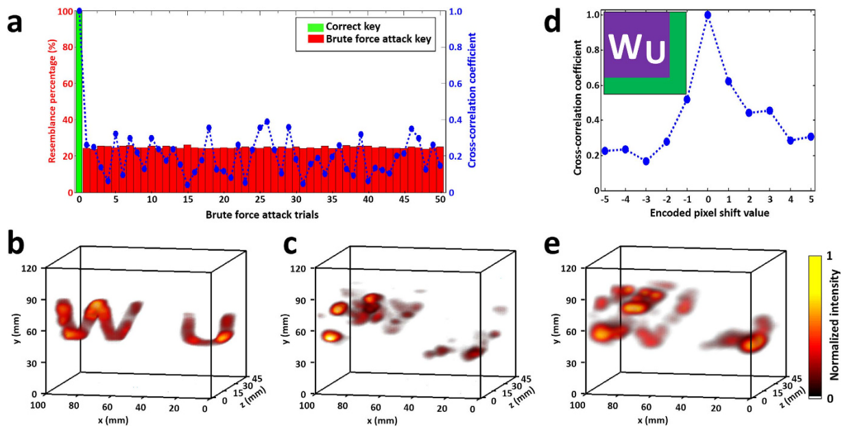
Figure 4. Security of the ToF-CUP camera against two types of decryption attacks. (a) Cross-correlation coefficients between the image decrypted using the correct decryption key and images using 50 brute force attacks with wrong pseudo-random binary masks. (b) 3D datacube of letters “W” and “U” decrypted using the correct decryption key. (c) As in (b), but using an invalid decryption key in the brute force attack (trial #26). (d) Cross-correlation coefficients between the reconstructed image decrypted using the correct decryption key and each image using a part of the correct decryption key with a different horizontal shift. Positive shift pixel numbers mean the key was shifted to the right of the acquired image, while negative numbers mean a shift to the left. The inset shows the relative positions of the letters “W” and “U” and the full decryption key (green). The part of the decryption key used in the shift security test is marked in purple. (e) As in (b) and (c), but using a part of the correct decryption key right shifted by one encoded pixel.
