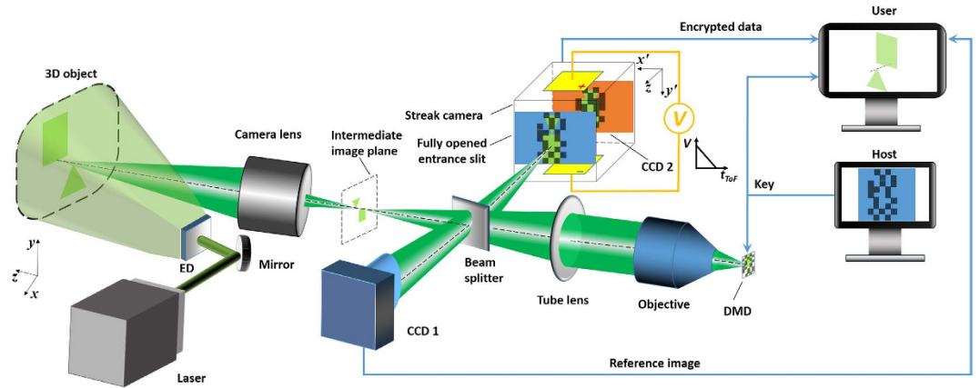
Figure 1. ToF-CUP system configuration. CCD, charge-coupled device; DMD, digital micromirror device; ED, engineered diffuser; V , sweeping voltage; t_{ToF} , time-of-flight. Equipment details: camera lens, Nikon, f = 18\text{--}55\text{ mm} ; CCD 1, Point Grey, FMVU-03MTM-CS; CCD 2, Hamamatsu, ORCA-R2; DMD, Texas Instruments, DLP LightCrafter 3000; engineered diffuser, Thorlabs ED1-S20-MD; laser, Attodyne, APL-4000; microscope objective, Olympus UPLSAPO 4 \times ; streak camera, Hamamatsu C7700; tube lens, Thorlabs AC254-150-A.
