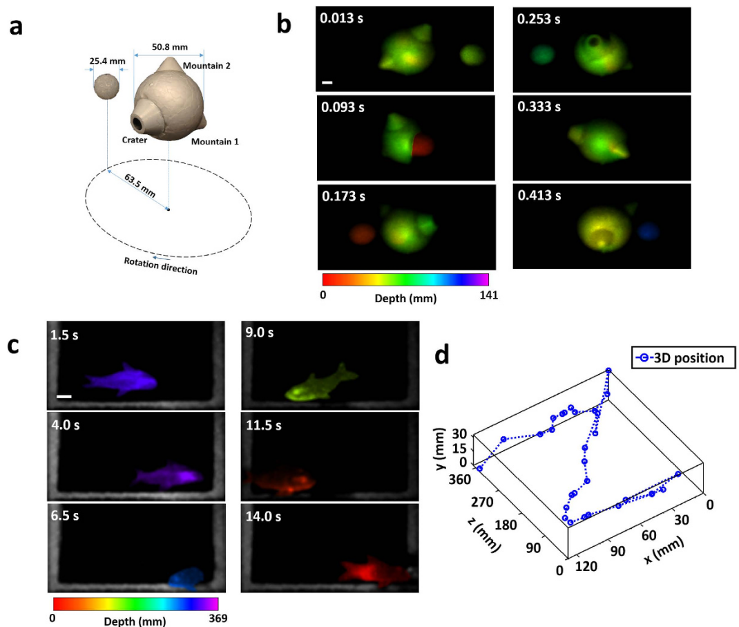
Figure 5. ToF-CUP of moving objects. (a) Experimental setup of two rotating balls. (b) Representative depth-encoded 3D images at six different slow-time points showing the relative depth positions of these two balls. The corresponding movie is in Supplementary Video 2. We also applied ToF-CUP imaging to a live comet goldfish. (c) Representative depth-encoded 3D images at six different slow-time points. (d) Trace of the 3D position of the fish. The corresponding movie is Supplementary Video 3. Scale bar: 10 mm.
