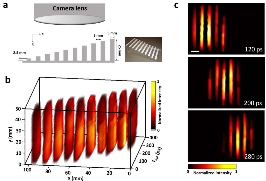
Figure 2. Quantification of ToF-CUP's depth resolution. (a) Side view and photograph of the height-varying fin-pattern target used in the experiment. The ToF-CUP system was placed perpendicularly to the target base and collected backscattered photons from the target surface. (b) Reconstructed x , y , t_{ToF} datacube representing the backscattered laser pulse intensity from the fins with different depths. (c) Representative x - y frames at t_{ToF} = 120 , 200, and 280 ps. Supplementary Video 1 shows the ToF snapshots of the x - y light distributions. Scale bar: 10 mm.
