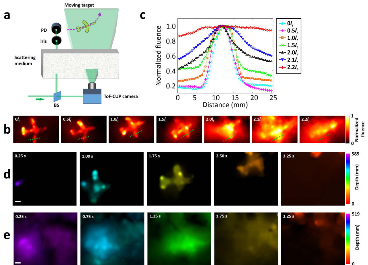
Figure 6. ToF-CUP imaging of an object moving behind a scattering medium. (a) Experimental setup. BS, beam sampler; PD, photodiode detector. The airplane moves from the lower left to the upper right, as well as toward the ToF-CUP camera in the depth direction. The trajectory of the airplane-model target is marked by the magenta dashed line with an arrow. (b) Projected images of the airplane-model target acquired at various scattering thicknesses of the scattering medium, where the projection was achieved by summing over the x , y , z datacube voxels along the z axis. (c) Comparison of the normalized fluence profiles of the airplane wing along the green dotted lines in (b). (d) Representative depth-encoded ToF-CUP images of an airplane target moving behind a scattering medium with an equivalent scattering thickness of 1.0l_t . (e) As in (d), but with an equivalent scattering thickness of 2.1l_t . The corresponding movie is Supplementary Video 4. Scale bar: 10 mm.
