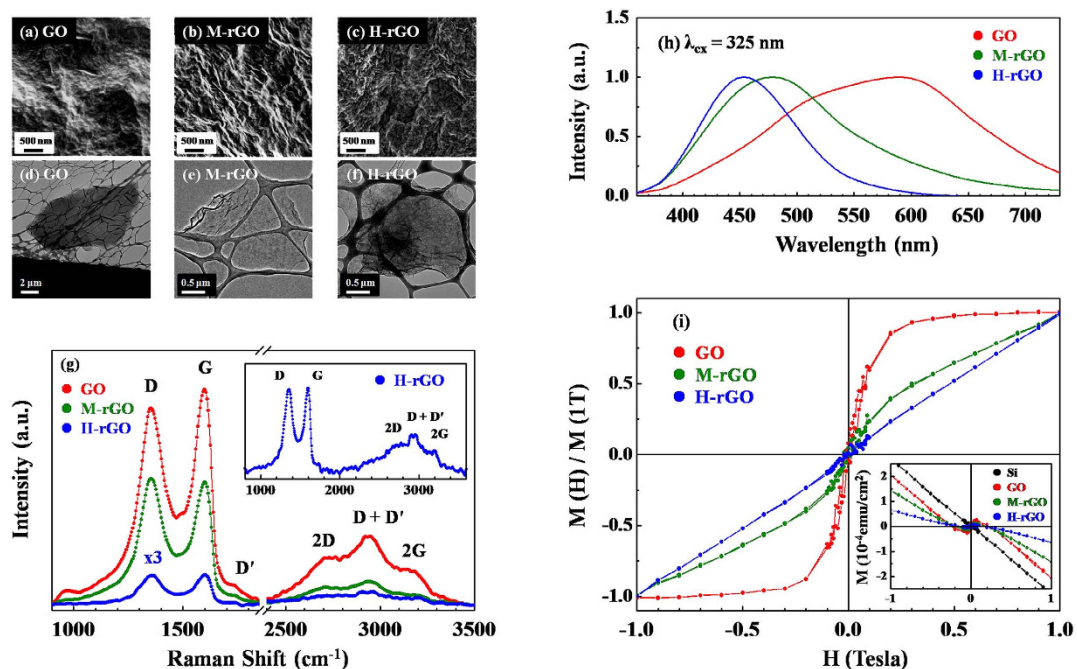
Figure 1. Field Emission Scanning Electron Microscopy images of (a) GO, (b) M-rGO and (c) H-rGO. Transmission Electron Microscopy images of (d) GO, (e) M-rGO and (f) H-rGO. (g) Raman spectra of GO, M-rGO and H-rGO; inset magnifies Raman spectrum of H-rGO. (h) PL spectra of GO, M-rGO and H-rGO. (i) Room-temperature [M(H)/M(1T)] -H curves of GO, M-rGO and H-rGO after subtraction of diamagnetic background that arises from silicon substrate. Inset in Fig. (i) plots M-H curves (without background subtraction) of GO, M-rGO and H-rGO.
