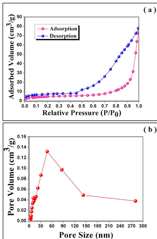
Figure 2. (a) Nitrogen adsorption-desorption isotherm curve of mesoporous TiO 2 hollow nanofibers. (b) Pore size distribution curve of the mesoporous TiO 2 hollow nanofibers.
