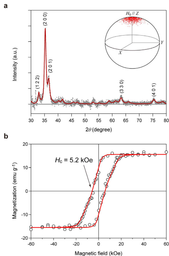
Figure 3. Crystallographically oriented nanometer-sized \epsilon -Fe 2 O 3 . (a) XRPD pattern of the crystallographically oriented S-1020 nanocrystal (average particle size = 8.2 nm) film. Grey dots and red line represent the observed and calculated patterns, respectively. The inset is the unit sphere illustration of the 3D distribution of the direction of the crystallographic a -axis of \epsilon -Fe 2 O 3 nanoparticles shown by red dots. The magnetic field was applied along the Z axis of the unit sphere. (b) The magnetic hysteresis loop of the crystallographically oriented S-1020 nanocrystal film measured in the applied magnetic field ( H_0 ) parallel to the easy-axis at 300 K. The red line is a guide to the eye.
