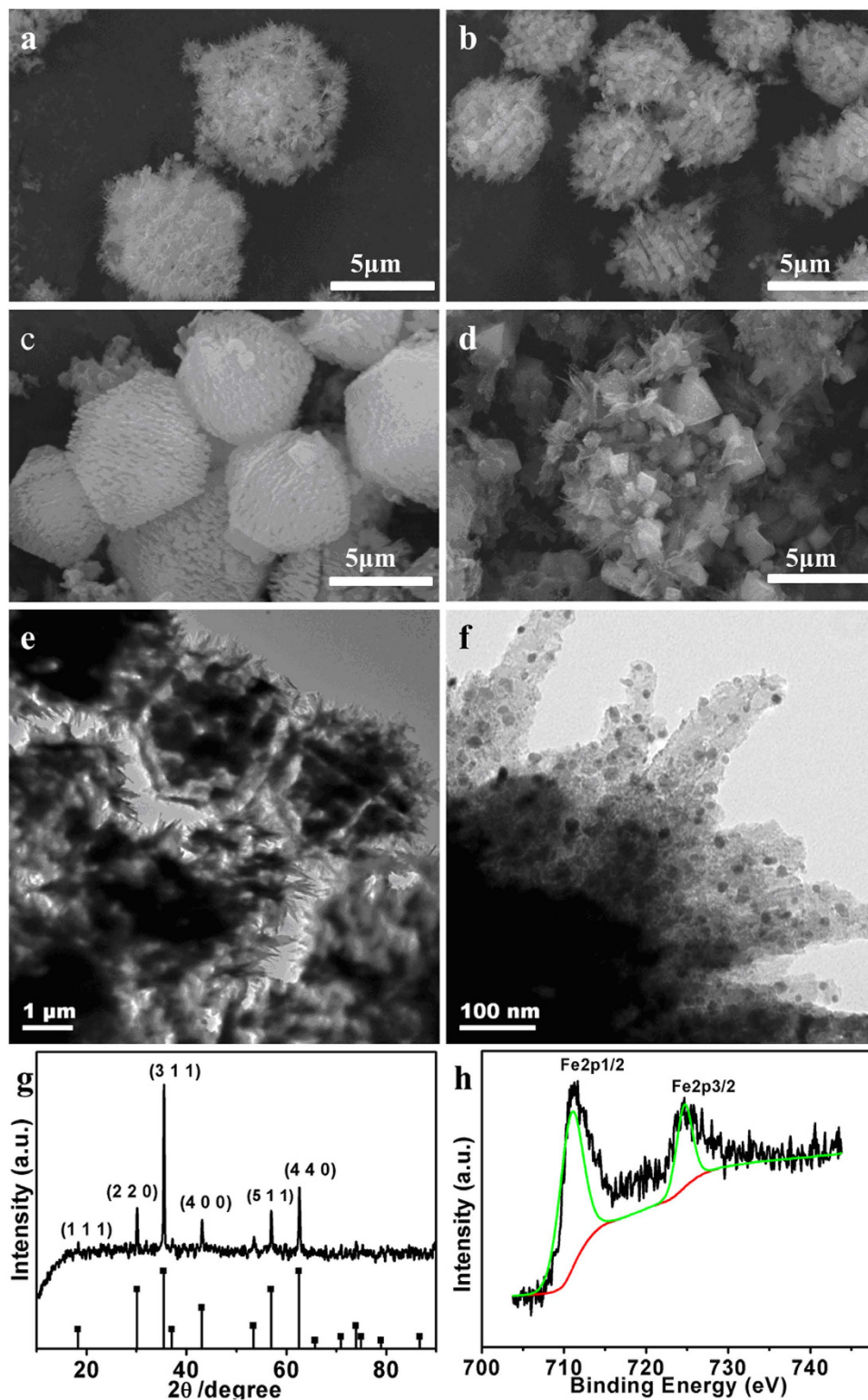
Figure 5. (a–d) SEM images of d-MIL-88A calcined at different temperature; 200 °C (a), 300 °C (b), 400 °C (c), 500 °C (d). (e,f) TEM images of \text{Fe}_3\text{O}_4@C_d by calcining d-MIL-88A at 400 °C. (g) XRD patterns of \text{Fe}_3\text{O}_4@C_d by calcining d-MIL-88A at 400 °C. (h) XPS of Fe 2p spectrum of \text{Fe}_3\text{O}_4@C_d derived from d-MIL-88A at 400 °C for 30 min.
