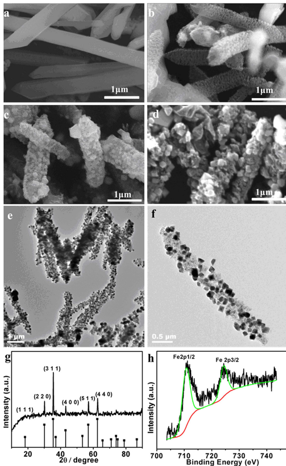
Figure 3. (a–d) SEM images of r-MIL-88A calcined at different temperature: 200 °C (a), 300 °C (b), 400 °C (c), 500 °C (d). (e,f) TEM images of \text{Fe}_3\text{O}_4@\text{C}_r by calcining r-MIL-88A at 400 °C. (g) XRD patterns of \text{Fe}_3\text{O}_4@\text{C}_r by calcining r-MIL-88A at 400 °C. (h) XPS of Fe 2p spectrum of \text{Fe}_3\text{O}_4@\text{C}_r derived from r-MIL-88A at 400 °C for 30 min.
