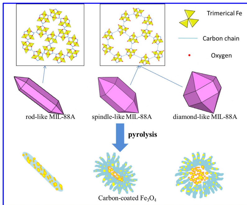
Figure 1. Schematic illustration of the formation process of Fe 3 O 4 @C nanostructures derived from MIL-88A.
