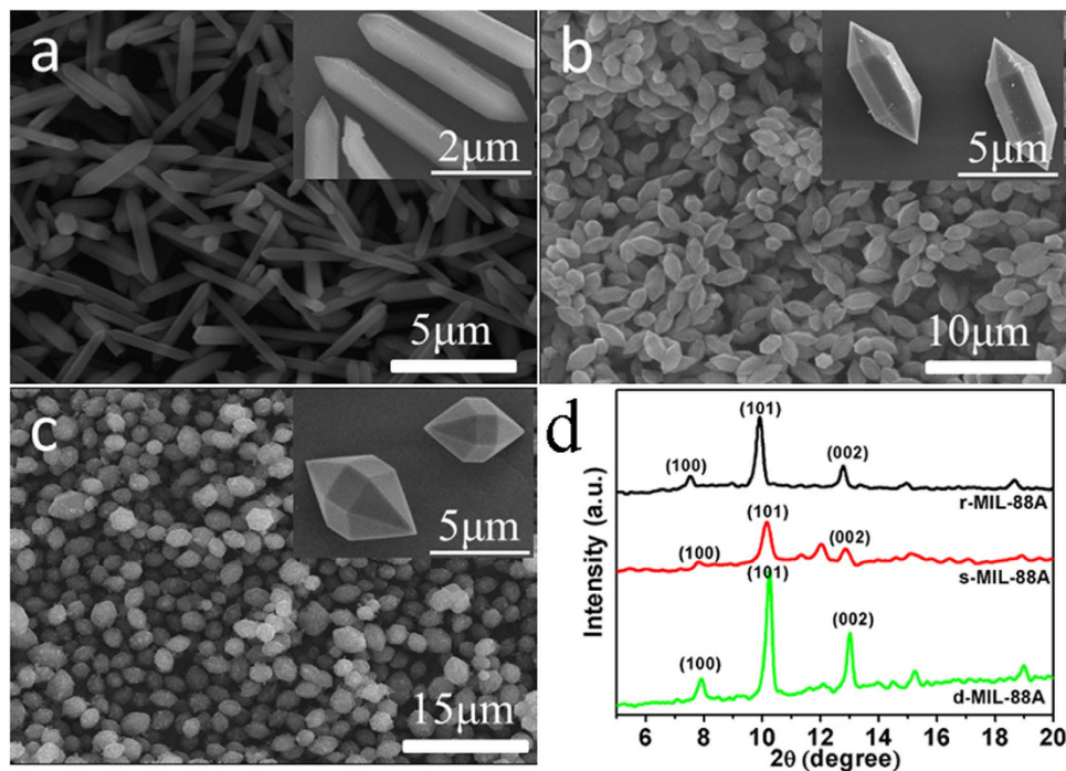
Figure 2. (a–c) SEM images of MIL-88A crystals with different structures: r-MIL-88A (a), s-MIL-88A (b) and d-MIL-88A (c). (d) XRD patterns of various MIL-88A: r-MIL-88A, s-MIL-88A and d-MIL-88A.
