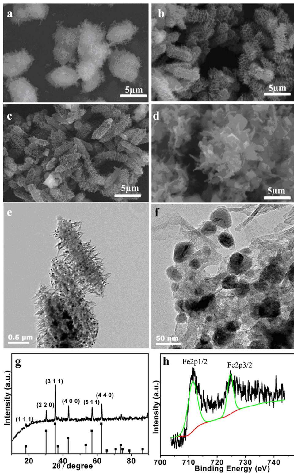
Figure 4. (a–d) SEM images of s-MIL-88A calcined at different temperature; 200 °C (a), 300 °C (b), 400 °C (c), 500 °C (d). (e,f) TEM images of Fe 3 O 4 @C s by calcining s-MIL-88A at 400 °C. (g) XRD patterns of Fe 3 O 4 @C s by calcining s-MIL-88A at 400 °C. (h) XPS of Fe 2p spectrum of Fe 3 O 4 @C s derived from s-MIL-88A at 400 °C for 30 min.
