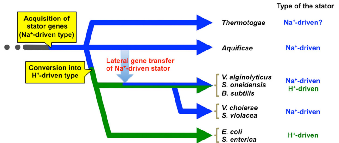
Figure 6. Schematic showing the acquisition and derivation of stator genes through bacterial evolution.
