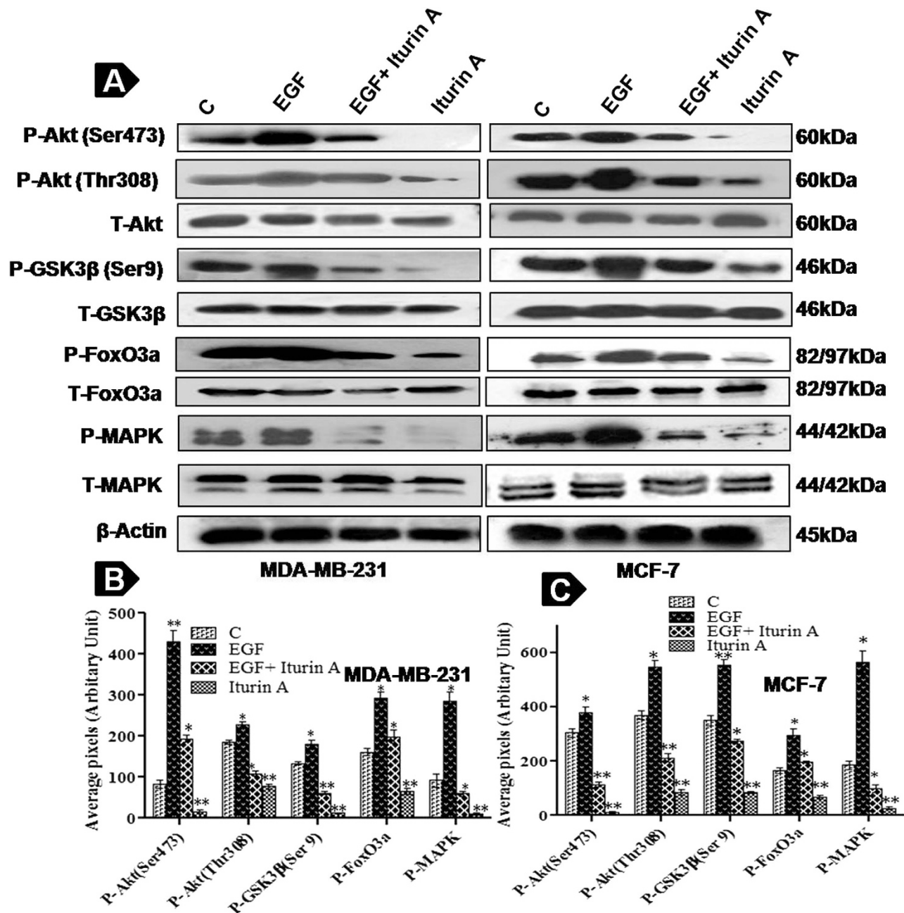
Figure 4. Iturin A inhibits Akt signaling pathway. (A) Phosphorylation levels of Akt (Ser473 and Thr308), GSK3 \beta , FoxO3a and MAPK (p44/42) are estimated along with corresponding total proteins expression in cells grown in serum-free medium and cells stimulated with recombinant human EGF (25 ng/ml) for 30 min alone and in the presence of Iturin A. Blots were cut and cropped according to the molecular weight of the proteins. (B) Graphical representation of phosphorylation level of Akt, GSK3 \beta , FoxO3a and MAPK in treated MDA-MB-231 cells. (C) Graphical representation of phosphorylation level of Akt, GSK3 \beta , FoxO3a and MAPK in treated MCF-7 cells. Data are represented as mean \pm S.D of three independent experiments. Significance level is represented by * P < 0.05 , ** P < 0.01 , *** P < 0.001 .
