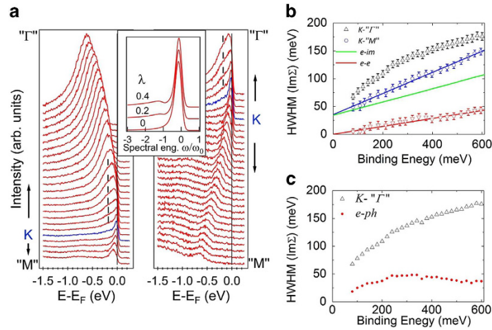
Figure 3. Original EDCs at 54 eV photon energy and the extracted quasiparticle widths. a, EDCs at 54 eV near the K point with each curve separated by 0.007 \text{ \AA}^{-1} . The phonon induced bump is highlighted. The inset shows the simulated spectral functions with an energy scale normalized to an Einstein phonon \omega_0 with various coupling constants. b, Extracted imaginary part of self energy (HWHM) along both K-\Gamma' and K-M' directions. c, Electron-phonon interaction extracted from K-\Gamma' branch.
