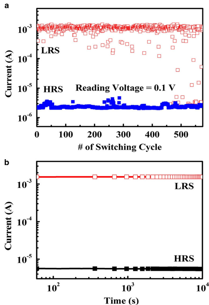
Figure 9. (a) Endurance and (b) retention properties of the thermal-baked albumen memory. The writing and erasing pulses are set to -1 V/100 ms and 2.5 V/100 ms, respectively, and a reading voltage of 0.1 V is applied.
